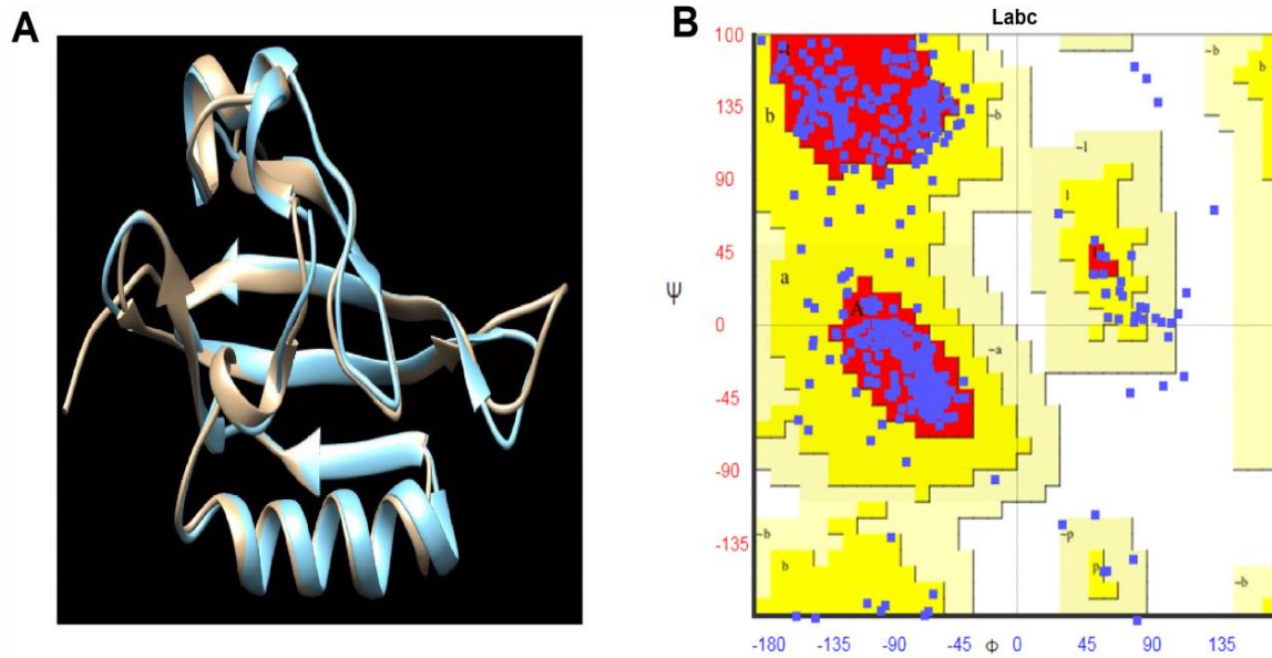
S1 Fig. In silico molecular modeling of mouse Ahr PAS-B domain. A) Superimposition of predicted 3D structure of mouse Ahr PAS-B domain with the human C-terminal PAS domain of HIF2a (PDB ID: 1p97). (B) Ramachandran plot of predicted mouse Ahr PAS-B domain.
