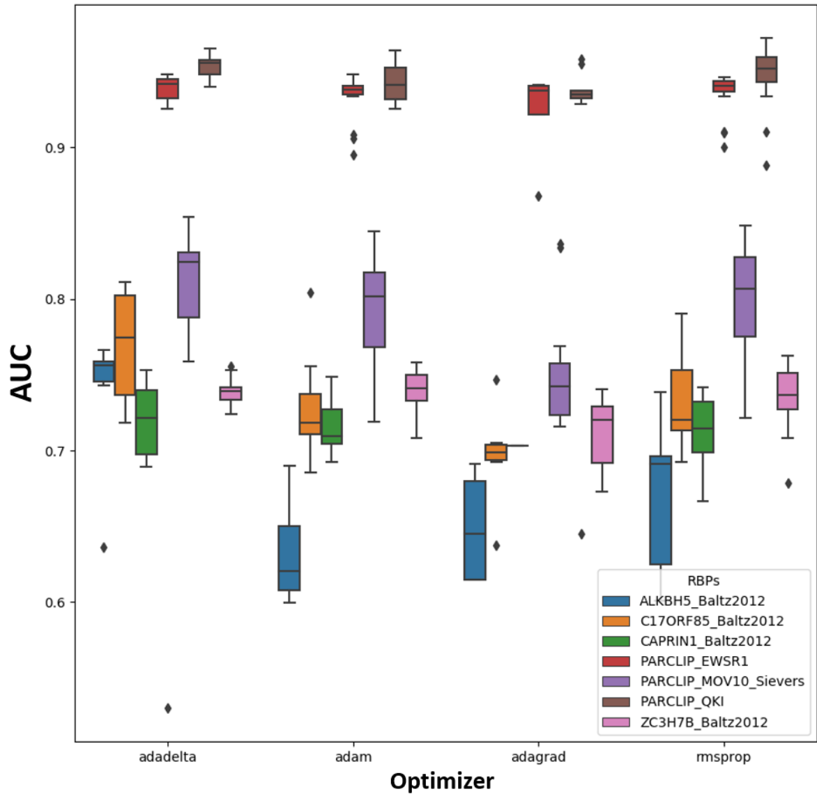
S7 Fig. mmCNN model optimization using 7 sample RBPs. For optimizer selection 5 sets of weight initialization range and 5 running rates for Adadelta, Adam, Adagrad, and Rmsprop optimizers.
