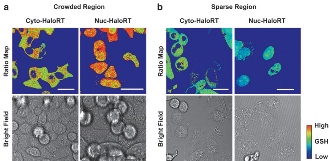
SUPPLEMENTARY FIG. S7. Representative ratio maps and bright field images of HeLa cells cultured in (a) crowded and (b) sparse region. The cells were either expressing nuc-Halo or cyto-Halo and were stained by HaloRT ligand. Scale bars are 10 \mu\text{m} .
