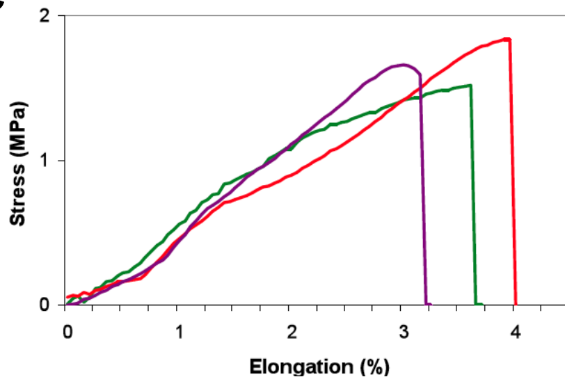
Fig. S1. SEM micrographs ( A ), histogram of fiber diameters ( B ) and examples of stress-elongation curves ( C ) of electrospun silk fibroin mats produced with 19% regenerated silk fibroin solutions.
