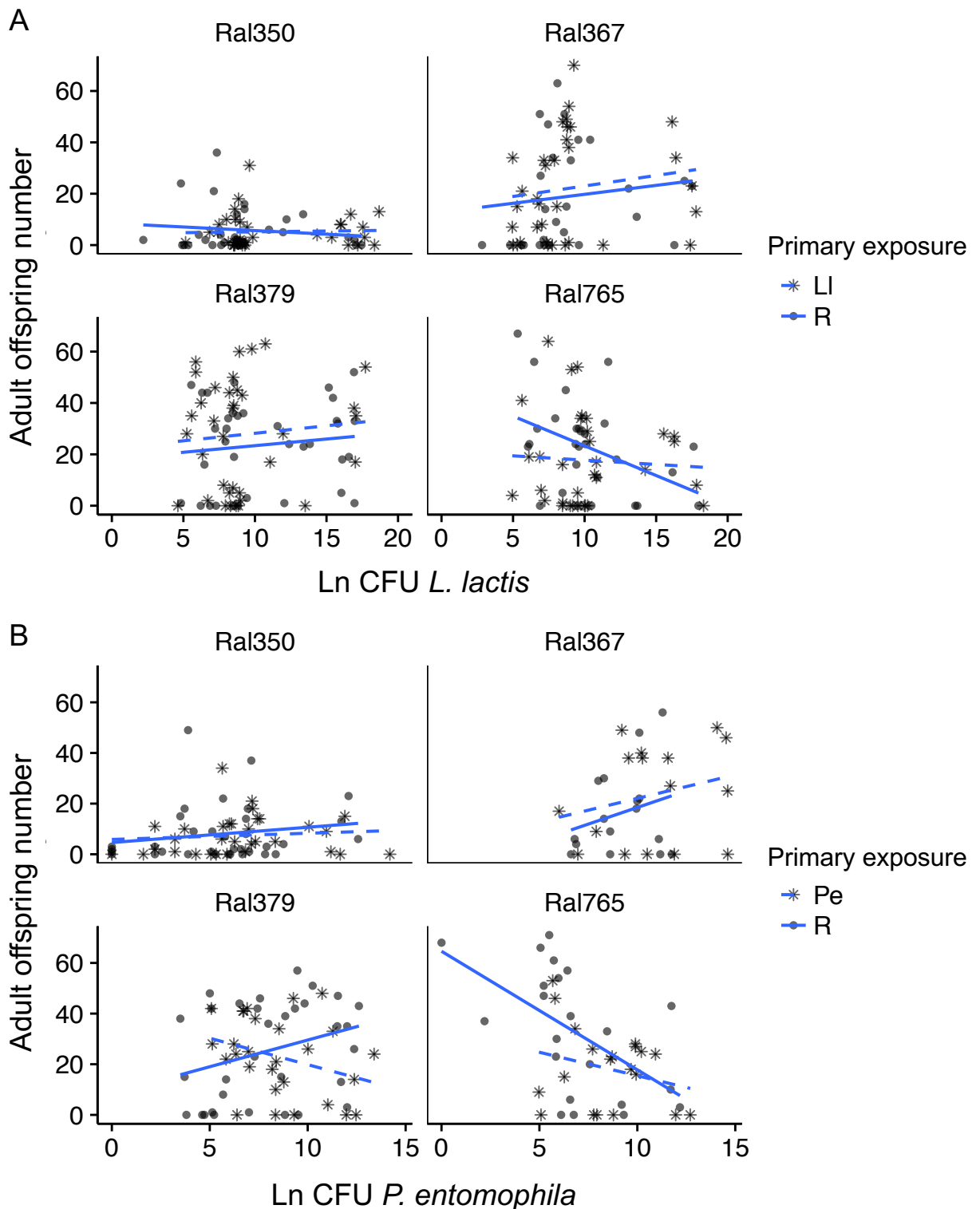
Fig. S4. Fecundity tolerance in relation to primary exposure and genotype 24 hours post challenge. Tolerance curves are plotted for each genotype and primary exposure-challenge treatment combination. (A) shows flies challenged with L. lactis and (B) shows flies challenged with P. entomophila .
