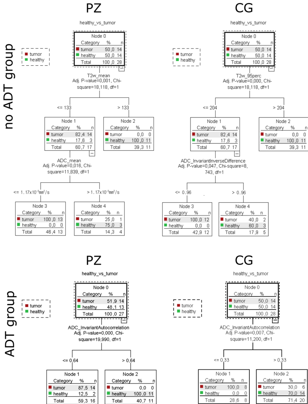
Figure S1 The decision tree diagrams for both patient groups and both healthy tissue ROIs.
