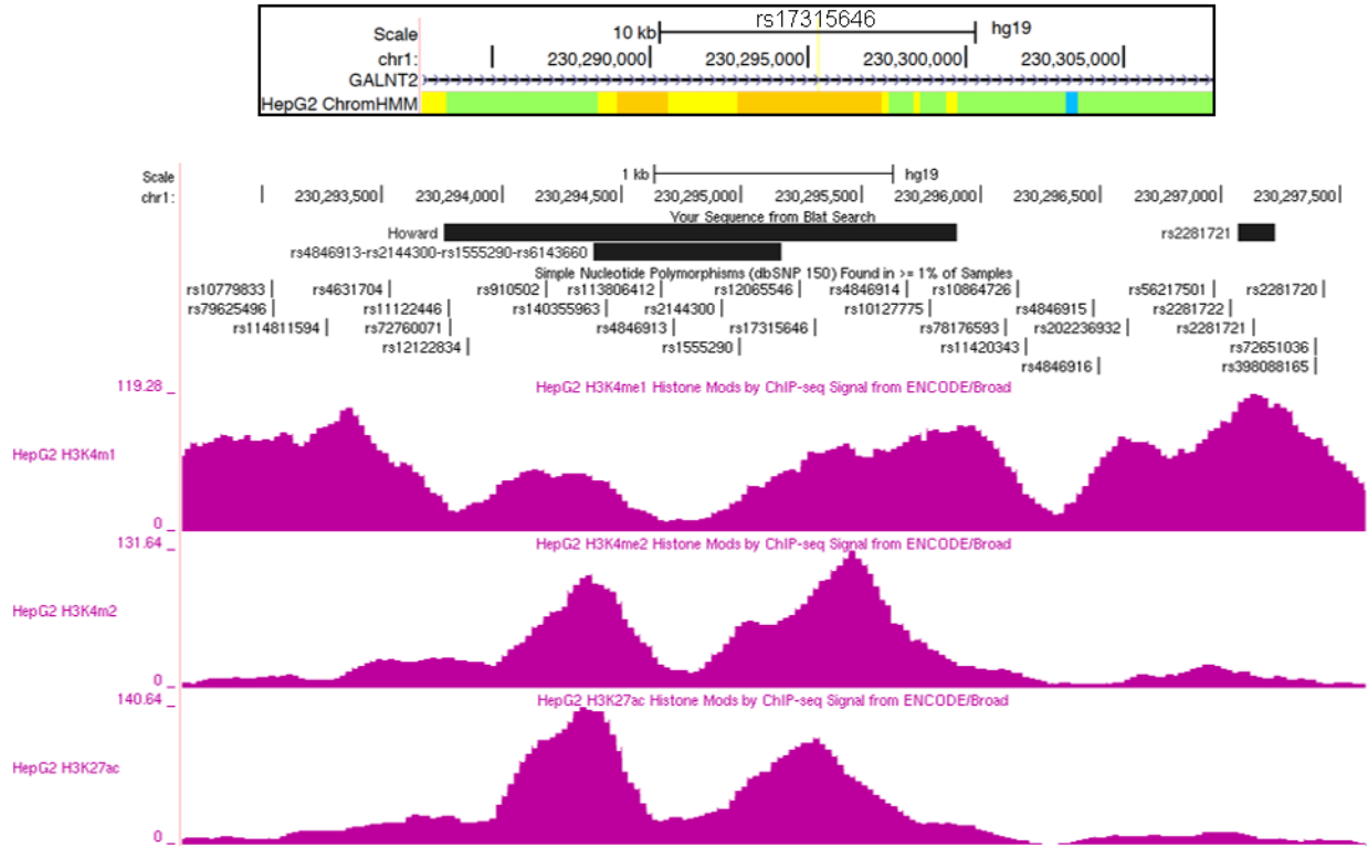
S8 Fig. Epigenetic landscape of the HDL-C associated region in GALNT2.
