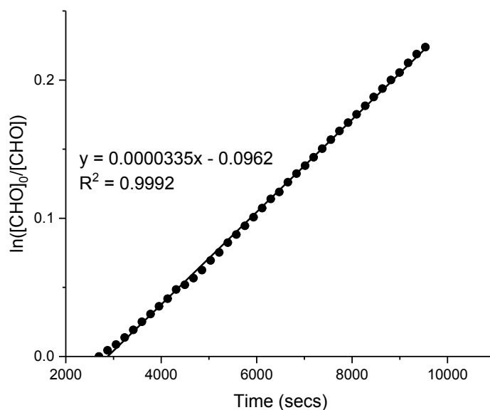
Figure S26 – Plot of \ln([CHO]_0/[CHO]) vs. time for CHO/CO 2 copolymerisation catalysed by 2f . The gradient of the graph represents k_{obs} , assuming a first order dependence on epoxide. Reaction conditions: 1:1000 catalyst:CHO, 80 °C at 1 bar CO 2 pressure. For clarity, only every 3 rd data point is shown.
