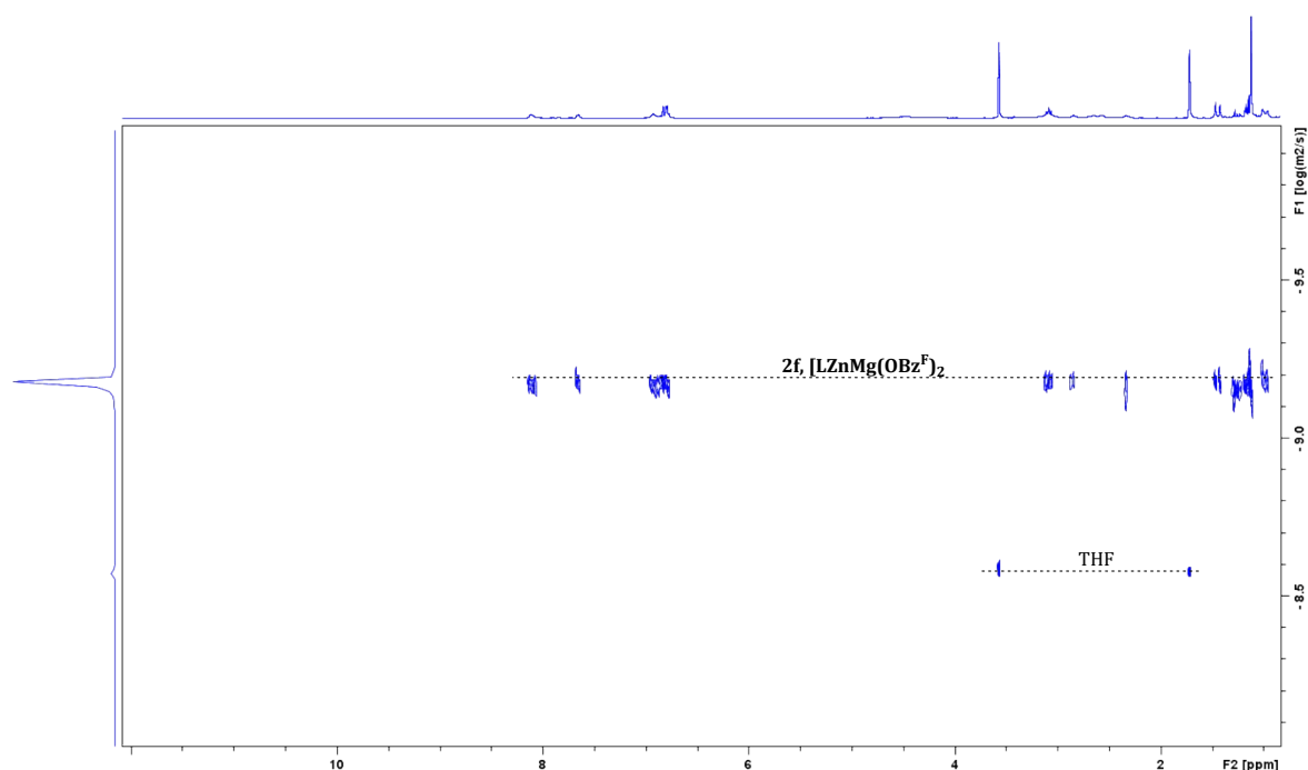
Figure S8 – DOSY NMR spectrum of complex 2f in d_8 -THF. Through comparison of the diffusion coefficient observed for 2f , to a calibration plot of known standards in d_8 -THF solution, 3 a predicted molecular weight of 938 \text{ g}\cdot\text{mol}^{-1} was obtained, in very close agreement with that of a monomeric species ( 919 \text{ g}\cdot\text{mol}^{-1} ).
