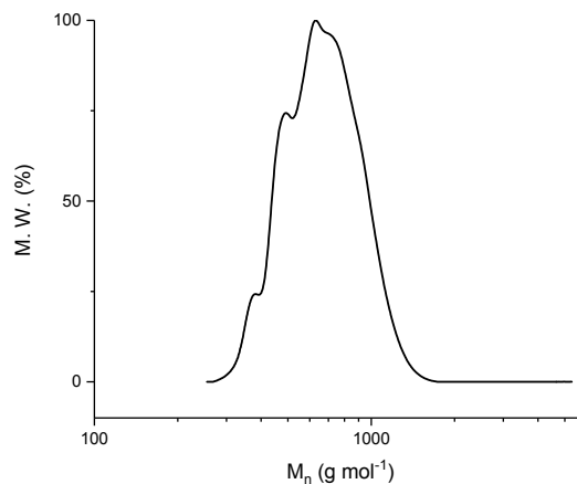
Figure S66 – SEC plot of M_n for catalyst 2b under 1 bar \text{CO}_2 . Reaction conditions: 2b /CHO/CHD = 1/1000/10, 80 °C, 5M in toluene. Conversion = 7.0 %.
