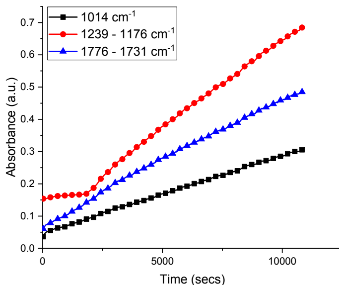
Figure S16 – ATR-IR spectroscopy plot showing the change in absorbance vs. time for three vibrational modes during the CHO/CO 2 copolymerisation catalysed by 2e . Reaction conditions: 1:1000 catalyst:CHO, 80 °C at 1 bar CO 2 pressure. For clarity, only every 10 th data point is shown
