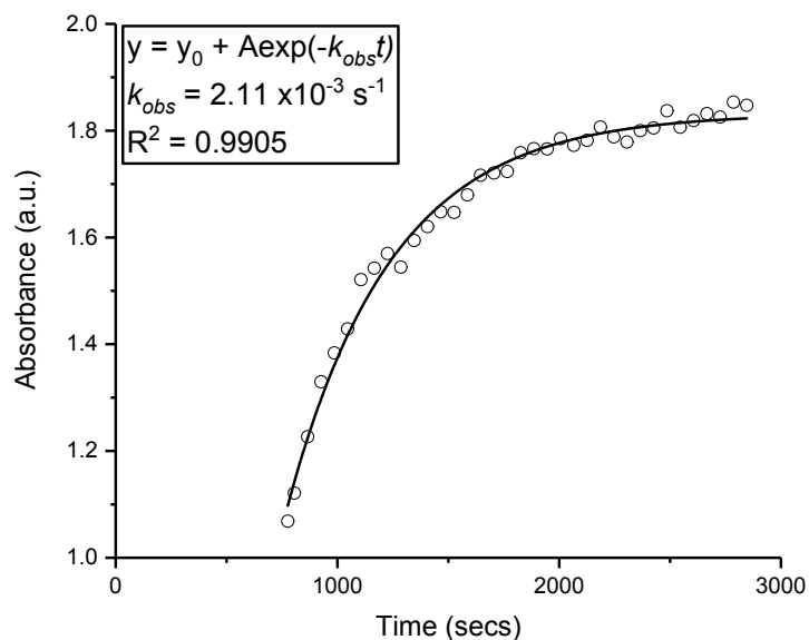
Figure S51 – ATR-IR spectroscopy plot showing the change in absorbance vs. time plot for the 1239-1176 \text{cm}^{-1} vibrational band, during the CHO/CO 2 copolymerisation catalysed by 2e . Reaction conditions: [CHO] 0 = 5 M in diethyl carbonate, [2e] 0 = 5 mM, 120 °C at 30 bar CO 2 pressure. For clarity, only every 2 nd data point is shown.
