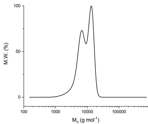
Figure S38 – SEC plot of M_n for catalyst 2h at 80 °C under 1 bar CO 2 for 6 hours.
