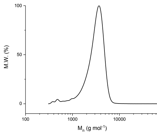
Figure S72 – SEC plot of M_n for catalyst 2b under 1 bar \text{CO}_2 . Reaction conditions: 2b /CHO/CHD = 1/1000/10, 80 °C, 5M in toluene. Conversion = 90.5 %.
