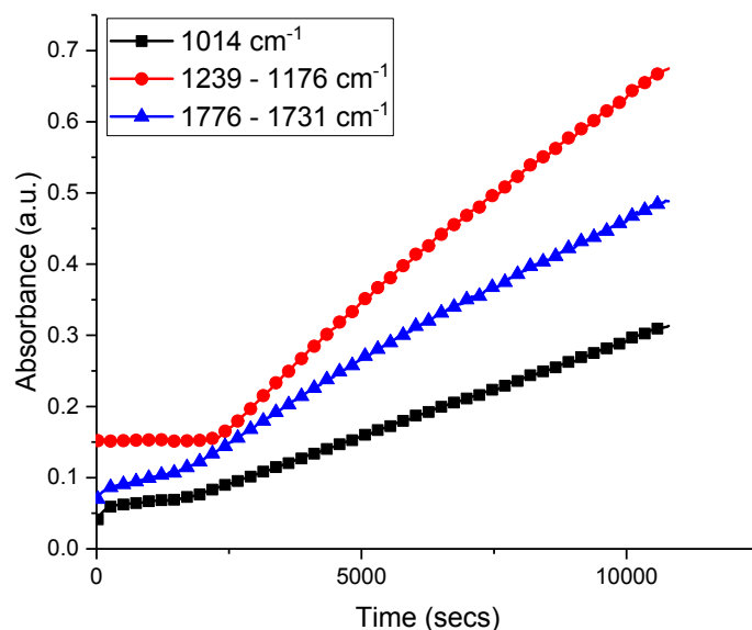
Figure S13 – ATR-IR spectroscopy plot showing the change in absorbance vs. time for three vibrational modes during the CHO/CO 2 copolymerisation catalysed by 2b . Reaction conditions: 1:1000 catalyst:CHO, 80 °C at 1 bar CO 2 pressure. For clarity, only every 8 th data point is shown.
