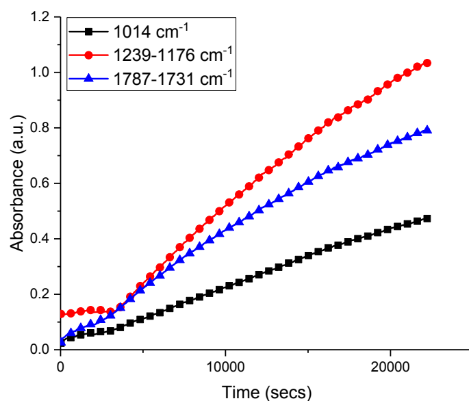
Figure S12 – ATR-IR spectroscopy plot showing the change in absorbance vs. time for three vibrational modes during the CHO/CO 2 copolymerisation catalysed by 2a. Reaction conditions: 1:1000 catalyst:CHO, 80 °C at 1 bar CO 2 pressure. For clarity, only every 20 th data point is shown.
