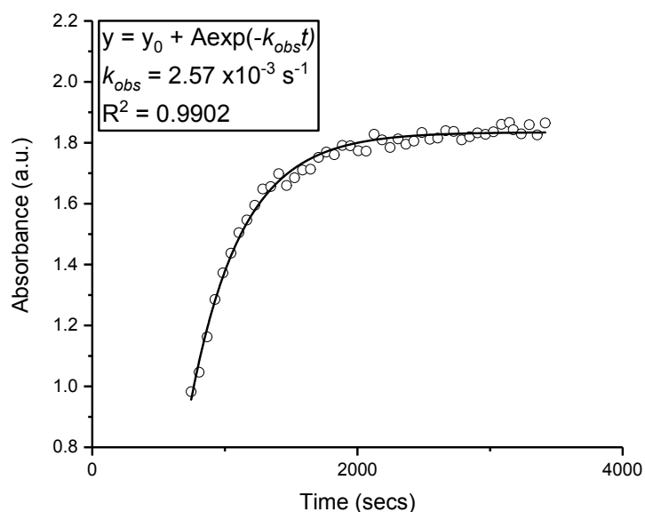
Figure S52 – ATR-IR spectroscopy plot showing the change in absorbance vs. time plot for the 1239-1176 \text{cm}^{-1} vibrational band, during the CHO/CO 2 copolymerisation catalysed by 2e . Reaction conditions: [CHO] 0 = 5 M in diethyl carbonate, [2e] 0 = 5 mM, 120 °C at 40 bar CO 2 pressure. For clarity, only every 2 nd data point is shown.
