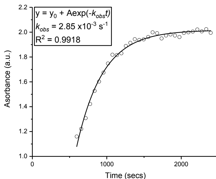
Figure S50 – ATR-IR spectroscopy plot showing the change in absorbance vs. time plot for the 1239-1176 \text{cm}^{-1} vibrational band, during the CHO/CO 2 copolymerisation catalysed by 2e . Reaction conditions: [CHO] 0 = 5 M in diethyl carbonate, [2e] 0 = 5 mM, 120 °C at 20 bar CO 2 pressure. For clarity, only every 2 nd data point is shown.
