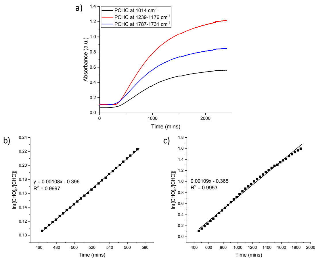
Figure S53 – a) ATR-IR spectroscopic trace of the copolymerisation of CHO and CO 2 . Reaction conditions: [1] = 5 mM and [CHO] 0 = 5 M in toluene, 80 °C, 1 bar pressure of CO 2 . b) Plot of \ln([CHO]_0/[CHO]) vs time for 10 to 20 % conversion of CHO. For clarity, every 2 nd data point is shown. c) Plot of \ln([CHO]_0/[CHO]) vs time for 10 to 80 % conversion of CHO. For clarity, every 20 th data point is shown.
