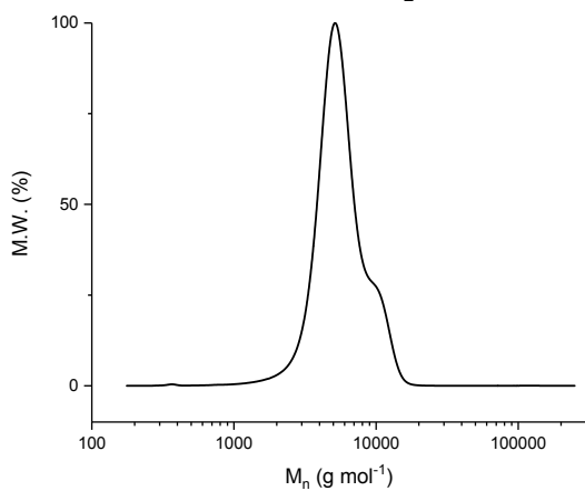
Figure S32 – SEC plot of M_n for catalyst 2b at 80 °C under 1 bar \text{CO}_2 for 3 hours.
