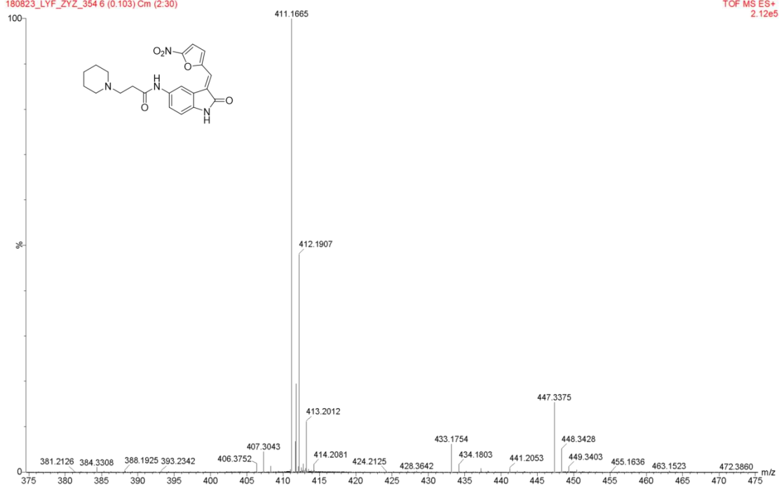
Figure S4. HRMS spectrum of compound ZY354
