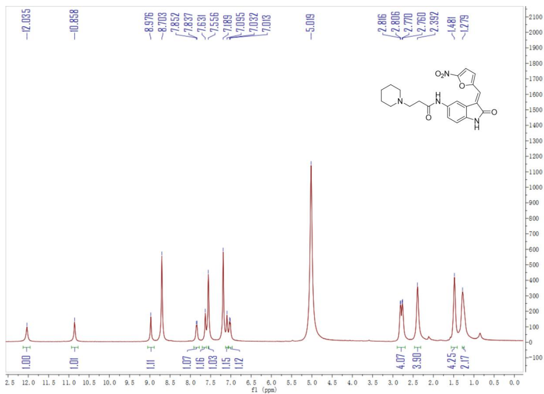
Figure S2. ^1\text{H} NMR spectrum of compound ZY354
