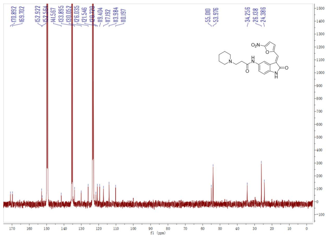
Figure S3. ^{13}\text{C} NMR spectrum of compound ZY354
