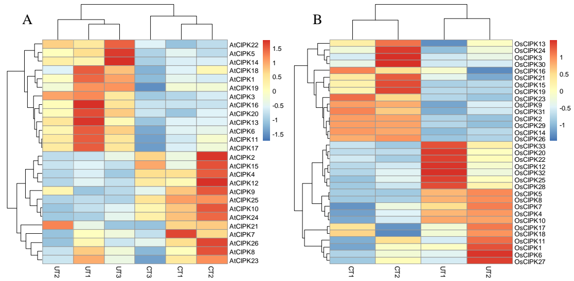
Supplemental Figure S6. Expression patterns of CIPK genes during cold stress. A, Expression patterns of CIPK genes in A. thaliana . B, Expression profiles of CIPK genes in O. sativa . CT, Chilling treatment; UT, Unchilling treatment.
