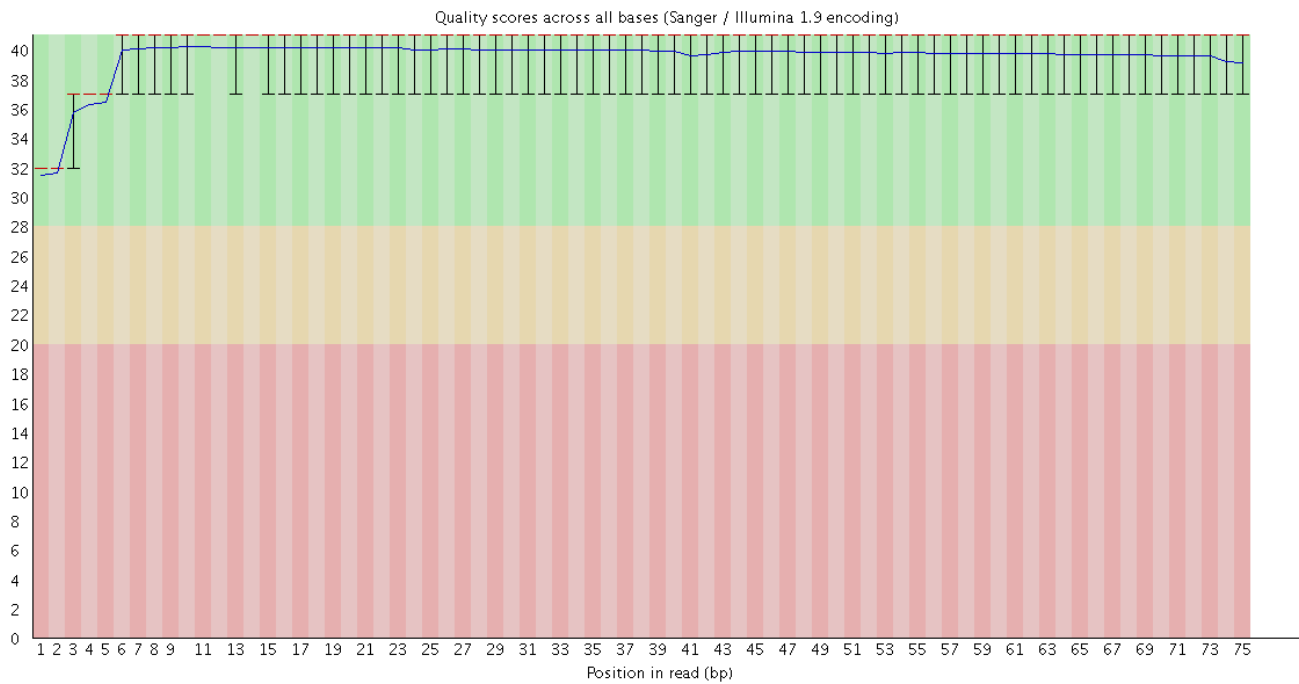
Supplementary Figure 2. Representative example of quality control of the sequencing reads obtained using FastQC. The y axis represents the mean quality score for each read position. Values in the green area are considered of good quality.
