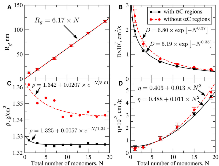
Figure 6. Molecular (Hydro)Dynamic Parameters for Double-Stranded Fibrin Polymers (with and without \alpha C Regions; Based on Data in Table 1)
