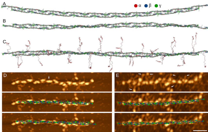
Figure 3. Comparison of Structures of Fibrin Protofibril FP 9/10 Obtained In Silico and In Vitro
