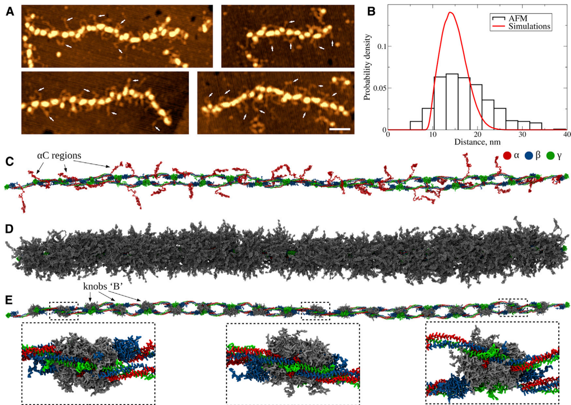
Figure 5. Dynamics of \alpha C Regions and Knobs “B”
