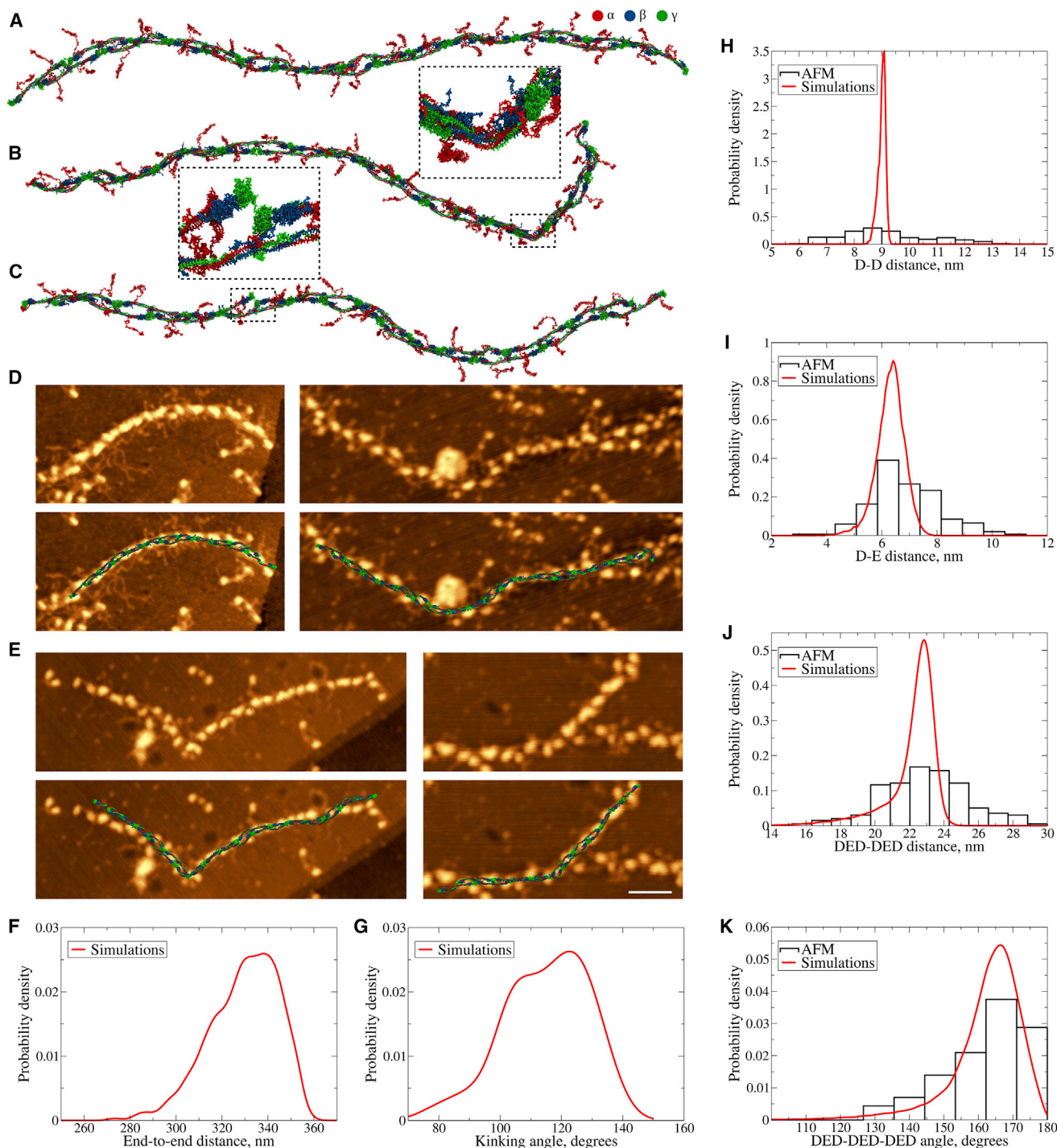
Figure 4. Conformational Dynamics of Fibrin Protofibrils
