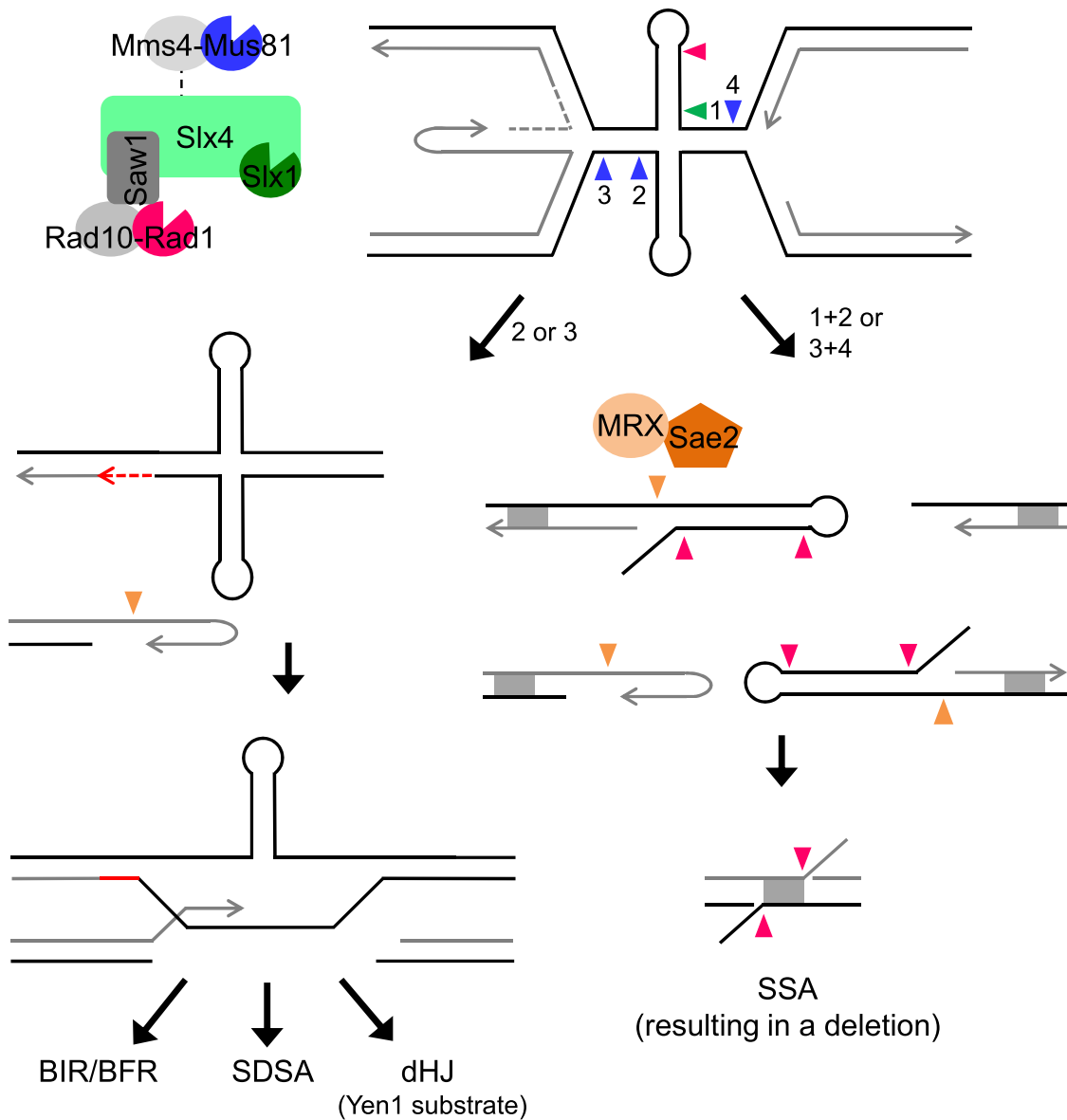
Figure 6. A Model for Mus81 and Six4 Complex Cleavage of Stalled Fork Substrates Formed by Secondary Structures at Flex1
