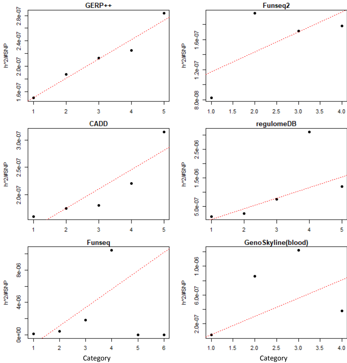
Supplemental Figure S1. Heritability per SNV ( h^2/\#\text{SNV} ) of HDL sorted by category of functional annotation score (TWINSUK cohort). Dashed lines represent linear regression results (categories merged).
