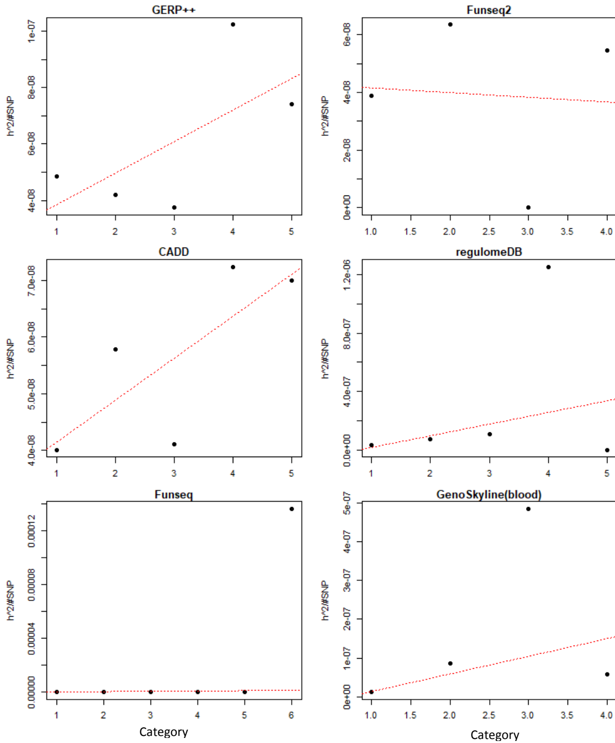
Supplemental Figure S3. Heritability per SNV ( h^2/\#\text{SNV} ) of BMI sorted by category of functional annotation score (TWINSUK cohort). Dashed lines represent linear regression results (categories merged).
