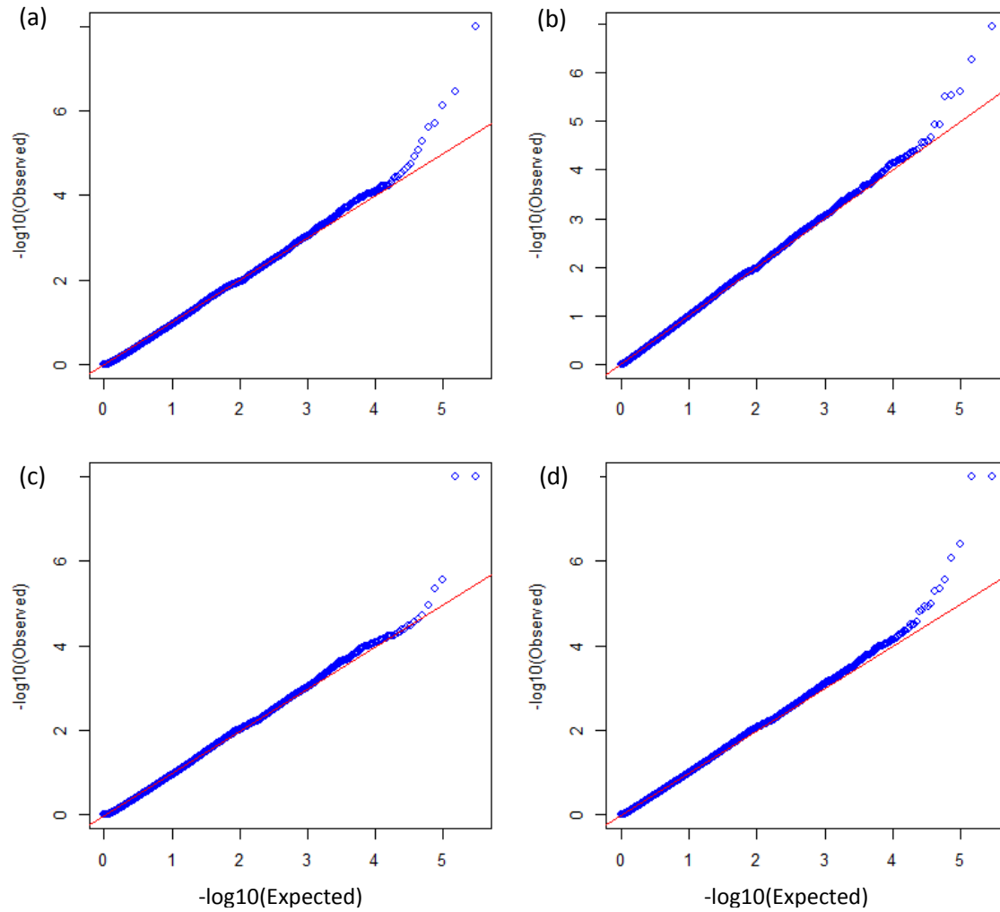
Supplemental Figure S9. Global QQ plots for association analysis of rare variants with BMI in the UK10K TWINSUK cohort: (a) FunSPU (genomic control \lambda = 0.604 ), (b) FunSPUw ( \lambda = 0.825 ), (c) wtFunSPU with global weights ( \lambda = 0.635 ), and (d) wtFunSPUw with global weights ( \lambda = 0.825 ).
