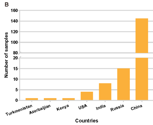
Supplemental Figure S1 | Spatio-temporal distribution of the VPI gene sequences from CVA4 strains available in GenBank. (A) Collection date; (B) Collection location.
