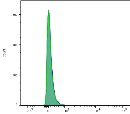
CD45
