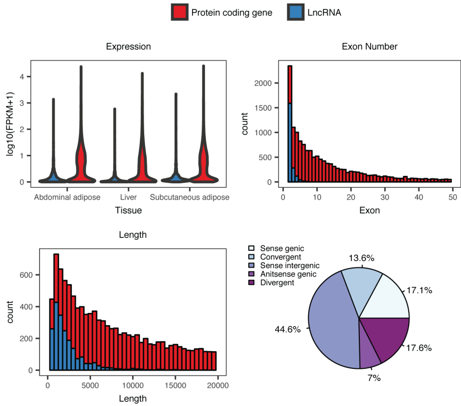
Figure S2. Comparison of characteristics of protein coding genes and lncRNAs and classification of lncRNAs.
