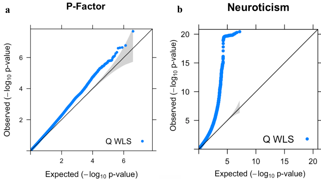
Supplementary Figure 14. Quantile-quantile plot for Q_{\text{SNP}} . Estimates are from WLS estimation for the p -factor (panel a) and neuroticism (panel b). Expected -\log_{10} p -values are those expected under the null hypothesis. The shaded area indicates the 95% confidence interval under the null. As some Q_{\text{SNP}} estimates for neuroticism were quite large, p -values < 5^{-20} were set to 5^{-20} .
