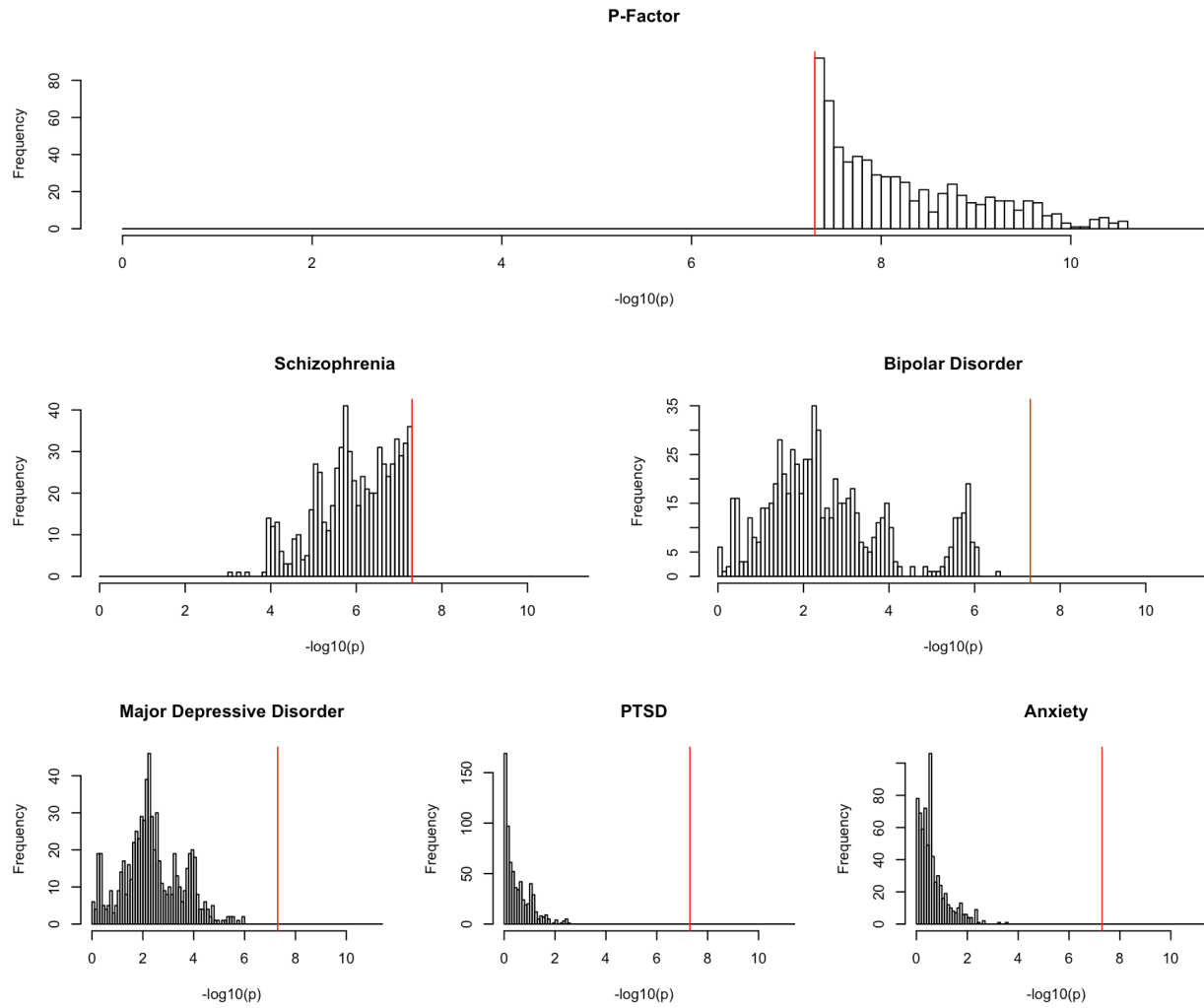
Supplementary Figure 12. Histograms of -\log_{10} p -values for hits on p -factor. Histograms of -\log_{10} p -values for the 684 non-independent SNPs that were genome wide significant for the p -factor using WLS estimation, but were not identified as significant in any of the individual GWASs. The vertical red line indicates genome wide significance.
