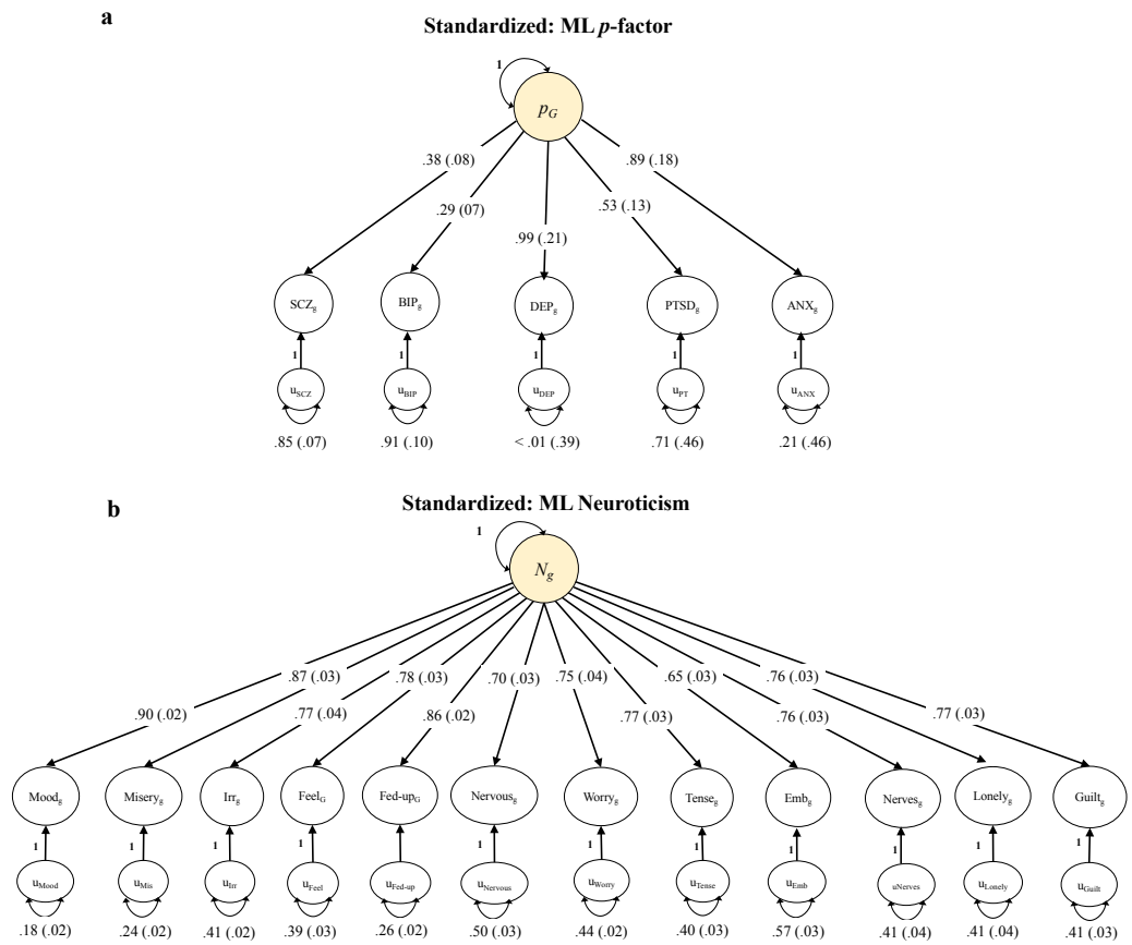
Supplementary Figure 24. ML estimates for neuroticism and p -factor Genomic SEM models.
