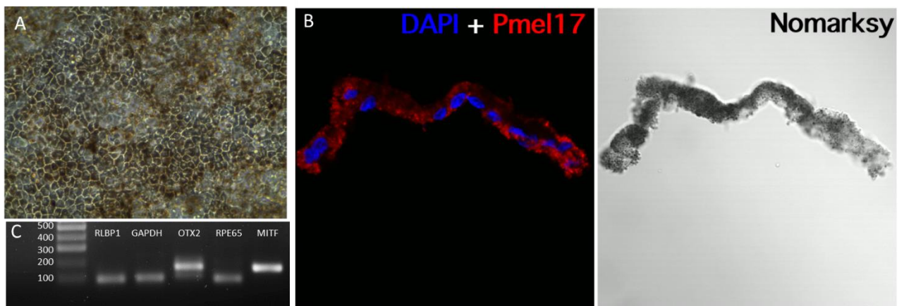
Figure S1: Characterisation of CHM Y42X patient derived iPSC-RPE. (A) Differentiated iPSC-RPE, displaying characteristic cobblestone morphology. (B) Immunostaining of iPSC-RPE sections stained for Pmel17 (red) and counterstained for DAPI (blue). (C) RT-PCR gel electrophoresis of RPE cell markers.
