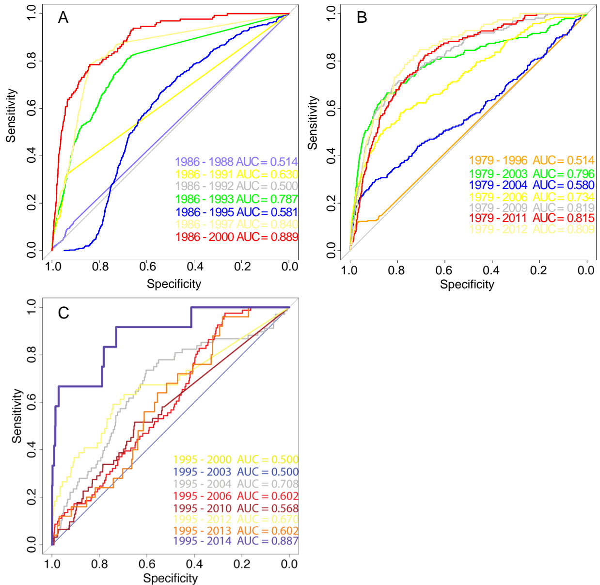
Supplementary Figure 7: Out of sample predictive accuracy as measured by Area Under the Curve (AUC) for Ae. albopictus in the United States (A) Ae. albopictus in Europe (B) and Ae. aegypti in the United States (C). Different colours represent different training datasets. Evaluation was always done on the subsequent set of data going forward to the last year of data.
