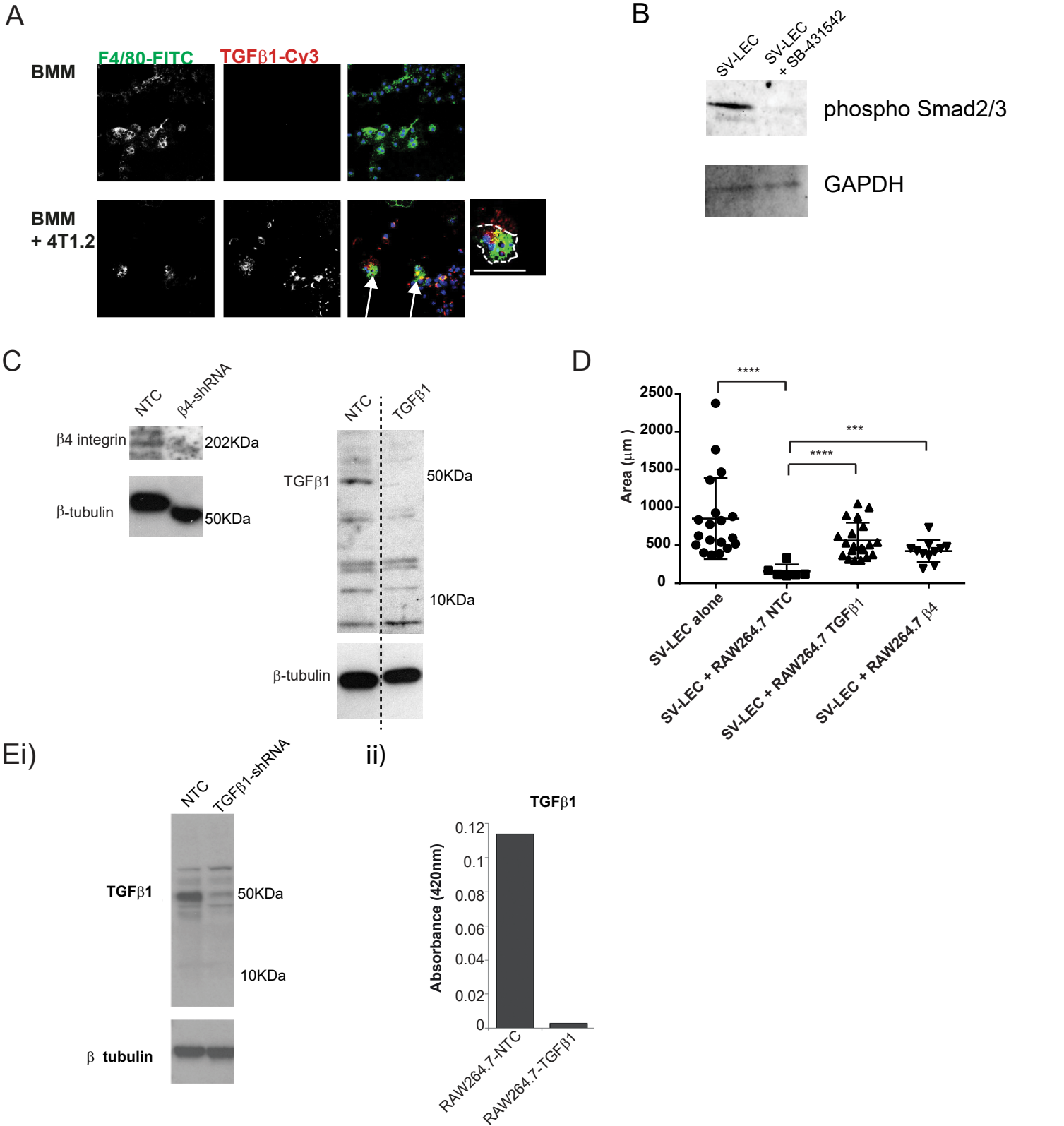
Figure S2. Western blot analysis of TGF \beta 1 knockdown in RAW264.7 cells, related to Figure 3 (A) Bone marrow macrophages were cocultured alone or with 4T1.2 tumor cells for 5 days on glass coverslips. Cells were fixed with 4% PFA before staining with F4/80-FITC and TGF \beta 1 and a Cy3 secondary antibody and imaging by confocal microscopy. Cell boundary depicted with white dotted line in inset image. (B) SV-LECs treated with SB-43142 were analysed by western blot to assess levels of phospho Smad2/3 (C) RAW264.7 were transiently transfected with shRNA against \beta 4 integrin or TGF \beta 1 and analysed by western blot. (D) Macrophages were cocultured with SV-LECs and the contraction of SV-LECs measured (E) RAW264.7 cells were virally transduced with shRNA against TGF \beta 1 or NTC. (i) Macrophages that were transfected were selected for GFP expression and lysed using an SDS buffer. Lysates were run on a reducing gel (4-12% Bis-Tris), blotted onto PVDF and the membranes were probed for TGF \beta 1 or \beta -tubulin as a loading control. (ii) Supernatants were analysed by ELISA for TGF \beta 1 levels.
