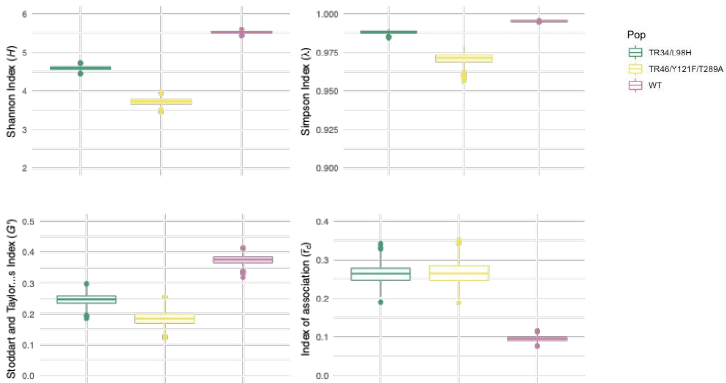
Fig S8: Clone-corrected genetic diversity indices of resistant Aspergillus fumigatus isolates harbouring either WT, TR34/L98H or TR46/Y121F/T289A CYP51A alleles.
