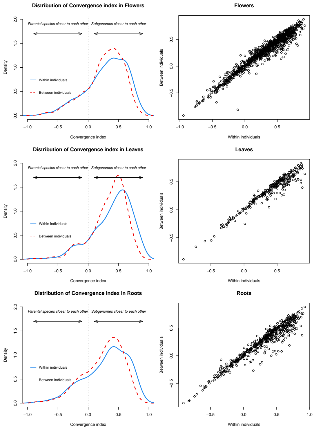
Fig. S6. Overall convergence indices estimated for C. bursa-pastoris subgenomes coming from the same individuals or from different individuals. The overall convergence indices, C , were computed from Cbp_{Co} and Cbp_{Cg} subgenomes expression levels from the same individuals (within individuals) or from different individuals (between individuals). The left panels show the distribution of C indices, and the right panels show the correlation between the two groups of estimates.
