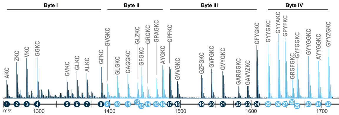
Figure S1. Spectrum of all 32 oligopeptides examined in this study. Oligopeptides were grouped by molecular weight into sets of eight, representing a byte of information (4 bytes total). The single-letter codes of residues in the information region are listed above each peak in the mass spectrum.
