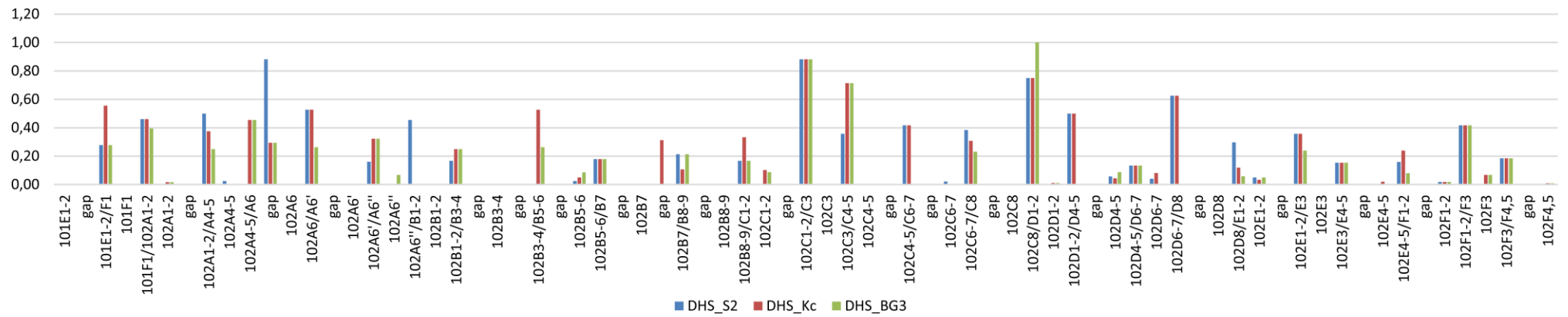
Fig. S21 The density of DNaseI hypersensitive sites (DHS) in the morphological structures of the fourth chromosome. The horizontal axis shows the bands and interbands of the fourth chromosome. The vertical axis shows the density of DHS (pcs/kb of the structure under consideration). Chart legend indicates the color code of cell line. Gaps correspond to model gaps which were not included in the bands or interbands.
