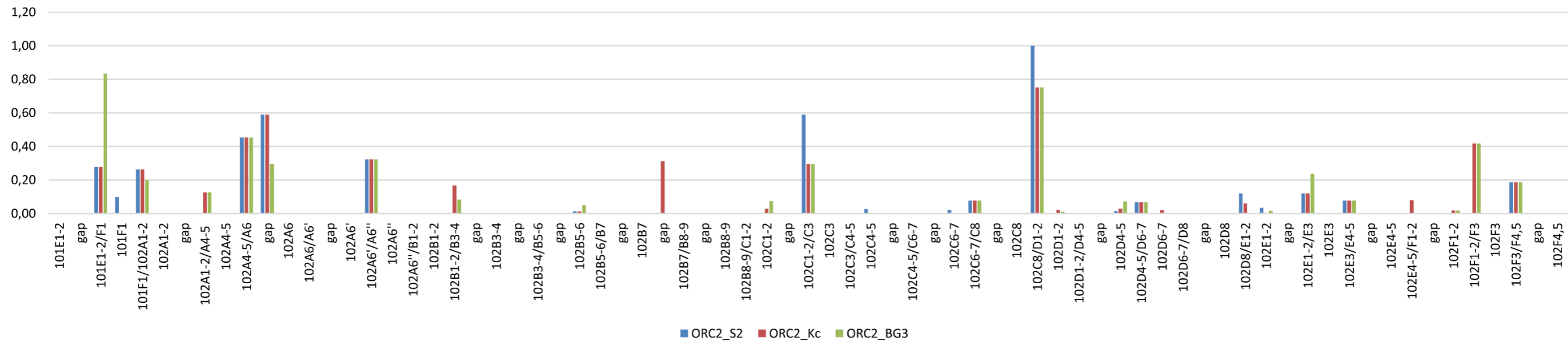
Fig. S18 The density of the ORC2 protein distribution in the structures of the fourth chromosome. The horizontal axis shows the bands and interbands of the fourth chromosome. The vertical axis shows the density of ORC2 binding sites (pcs/kb of the structure under consideration). Chart legend indicates the color code of cell line. Gaps correspond to model gaps which were not included in the bands or interbands.
