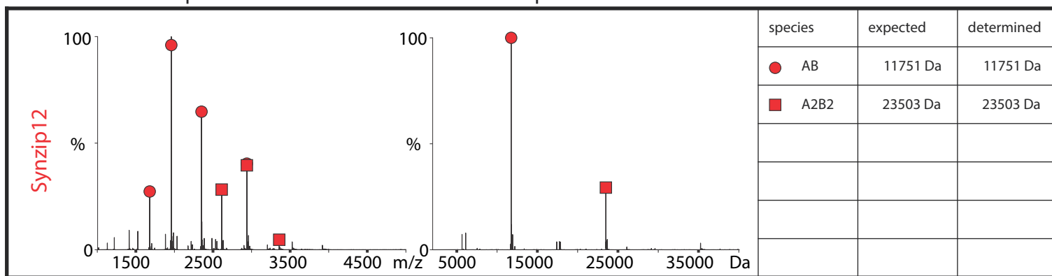
Mass spectrum
