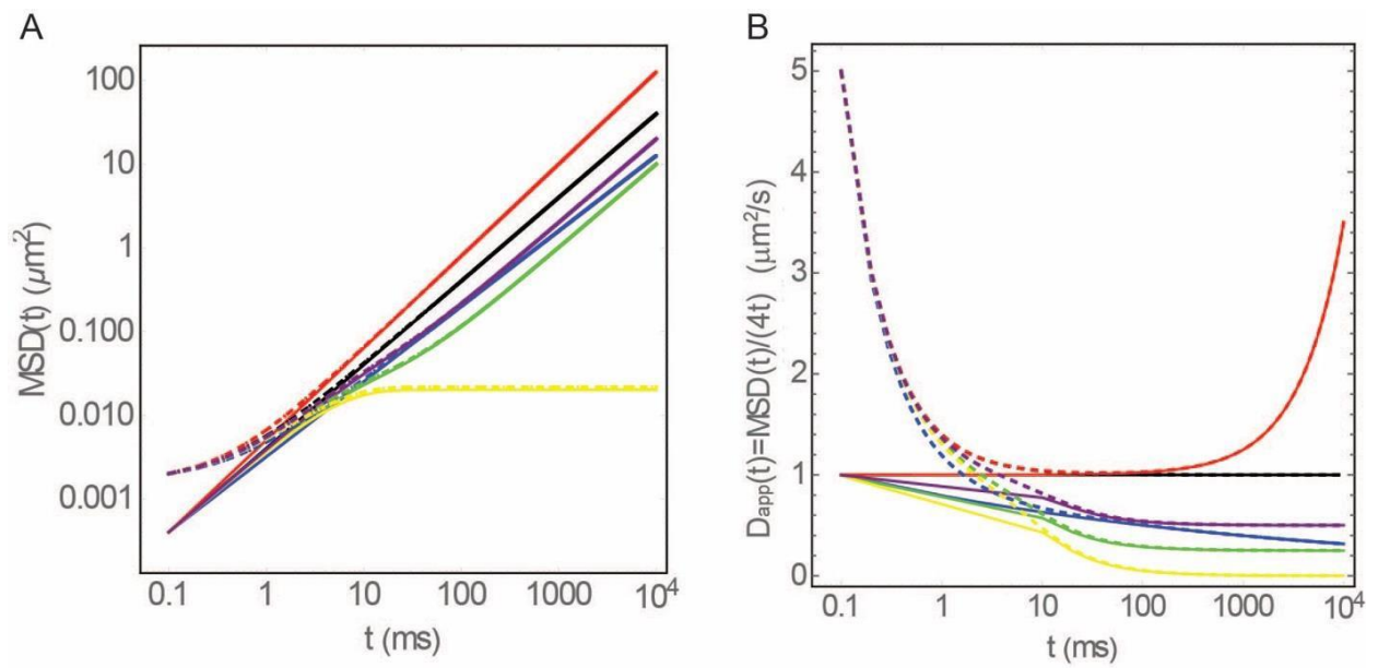
Supplemental Figure 2. Effect of spatial measurement error on the appearance of MSD versus time and MSD/(4t) versus time plots. Related to Figure 2.
