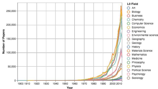
Figure 20. LO Fields-of-Study Number of Papers over Time. The numbers of papers in each field of study have increased drastically.
