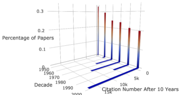
Figure 10. Citation Distributions over Time. The citation distributions of different decades show notable changes.
