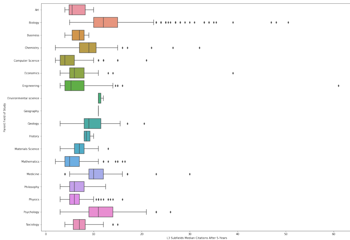
Figure S35. L3 Fields-of-Study Median 5-Year Citation Distributions by Parent Fields. We can observe the high variance among the L3 fields-of-study median citation numbers.
