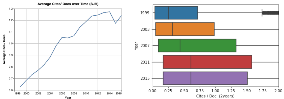
Figure 16. The Average Number of Citations ( \frac{Cites}{Docs} (2 years)) over Time. The average number of citations values have almost doubled in the last 18 years; additionally, their distributions have changed considerably.
