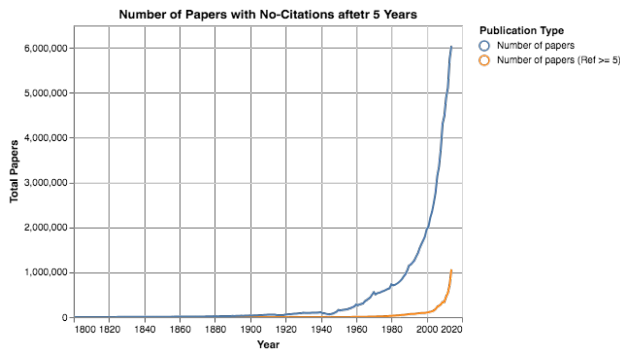
Figure 9. Total Number of Papers with No Citations after 5 Years. The number of papers with increased sharply over time.
