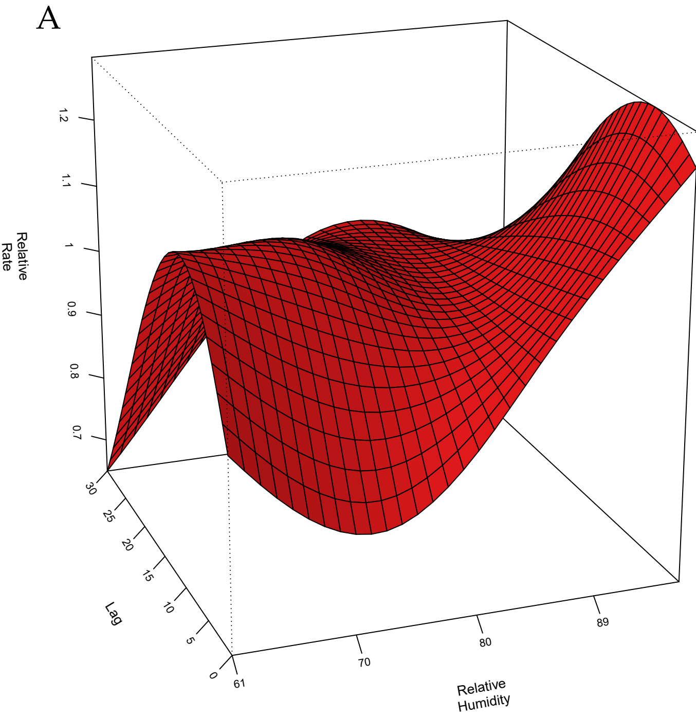
3D graph of Relative Humidity effect
