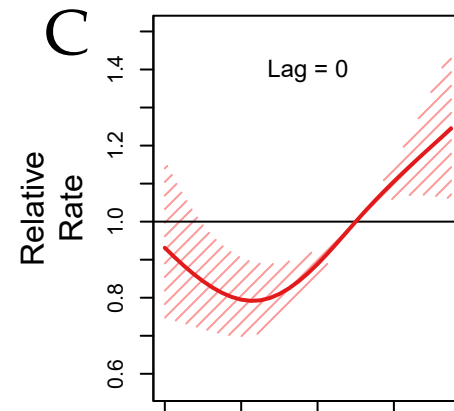
Slices in lag dimension
