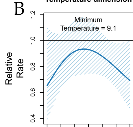
Slices in Minimum Temperature dimension
