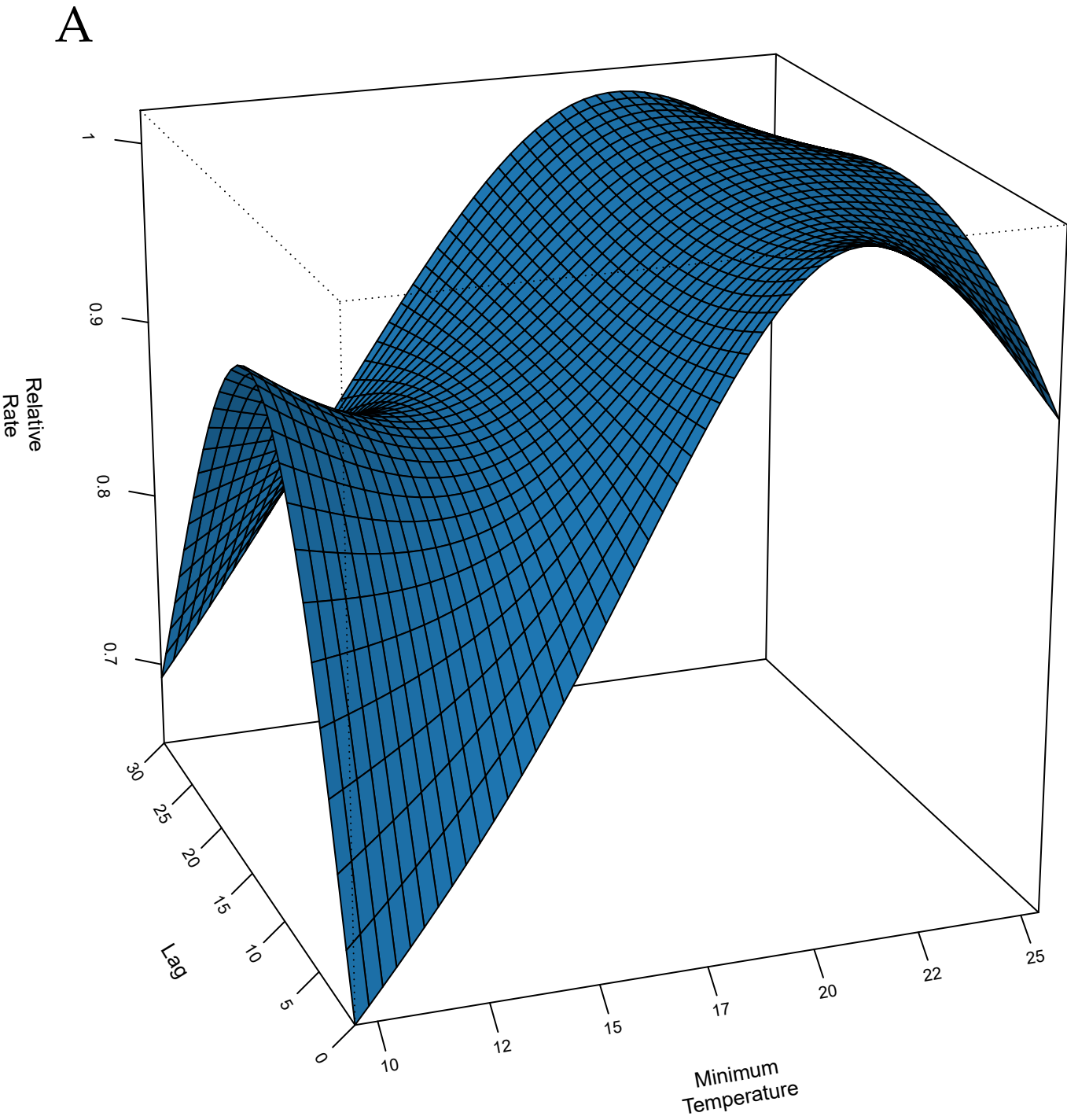
3D graph of Minimum Temperature effect
