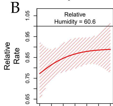
Slices in Relative Humidity dimension
