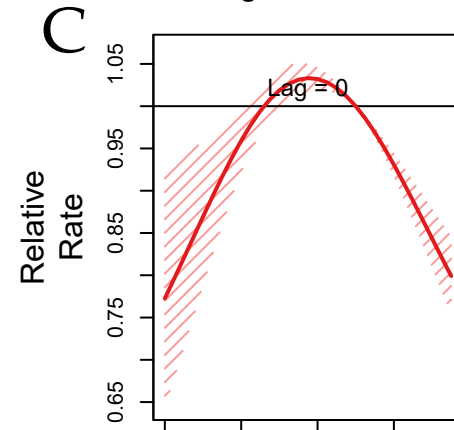
Slices in lag dimension
