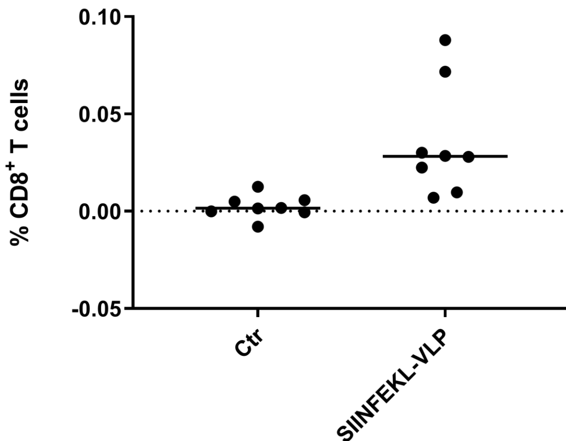
Figure S3. Cytokine production of SIINFEKL responsive CD8 + T cells. T-cells were stimulated with SIINFEKL peptide for 6 hours. The amount of INF \gamma and TNF \alpha double-positive cells is shown as percentage of total CD8 + T cells. Samples analyzed in this assay have been obtained from the same animal experiment described in Figure 7, with “Ctr” and “SIINFEKL-VLP” denoting the multiple vaccinations involving buffer-solution and OVA-replicon-VLP, respectively.
