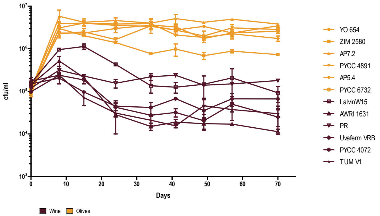
SUPPLEMENTARY FIGURE S1. Two replicate assays of growth and survival in olive brine of representatives of the Olives and Wine populations of S. cerevisiae .
