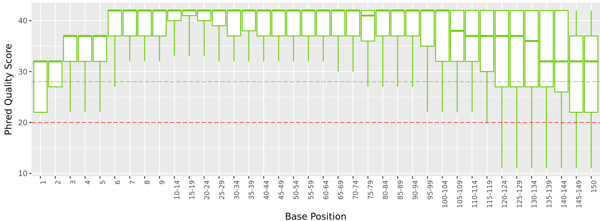
Gs-R2: Base Quality Distribution
