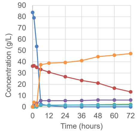
SS91 ( LpXI-E114G )
