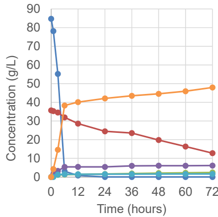
SS88 ( LpXI-N223I )
