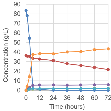
SS85 ( LpXI-Y13H/D228V )
