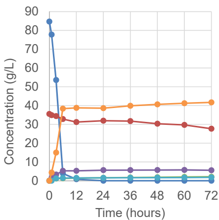
SS94 ( LpXI-L304S )
