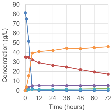
SS87 ( LpXI-D207G )
