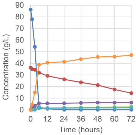
SS84 ( LpXI-K136T/A176T )
