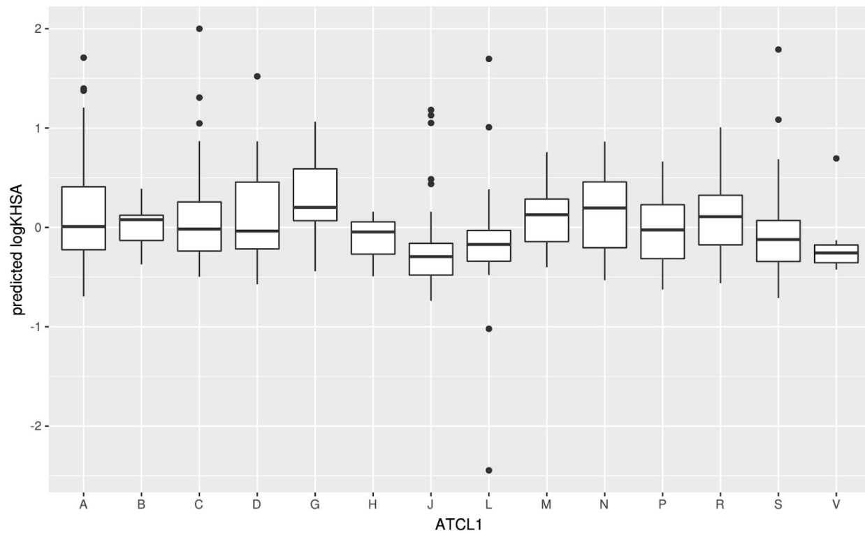
Fig S4: Predicted \log K_{\text{HSA}} values for the external 799 compounds in the CMap dataset grouped by ATC code level 1.
