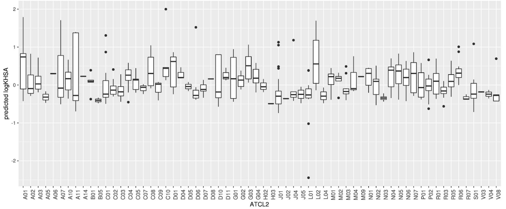
Fig S5: Predicted \log K_{HSA} values for the external 799 compounds in the CMap dataset grouped by ATC code level 2.
