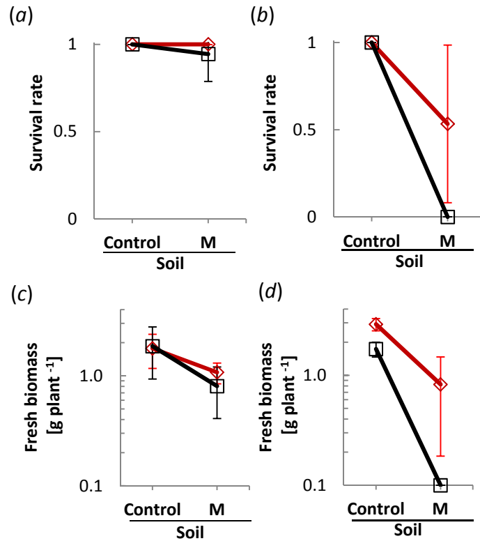
Figure S3. Independent experiment addressing local adaptation to metalliferous soil. (a,b) Survival of A. halleri (a) and A. arenosa (b) plants originating from Mias (M site, red colour) and Zapa (NM site, black colour) transferred into metalliferous (Mias) or non-metalliferous (control) soil. (c,d) Fresh biomass of A. halleri (c) and A. arenosa (d) plants originating from Mias (M site, red colour) and Zapa (NM site, black colour) transferred into metalliferous (Mias) or non-metalliferous (control) soil. Shown are means and standard deviation of survival rate (a,b) and fresh above-ground biomass (c,d) after 6 w of cultivation on experimental soils (see table S4 for details).
