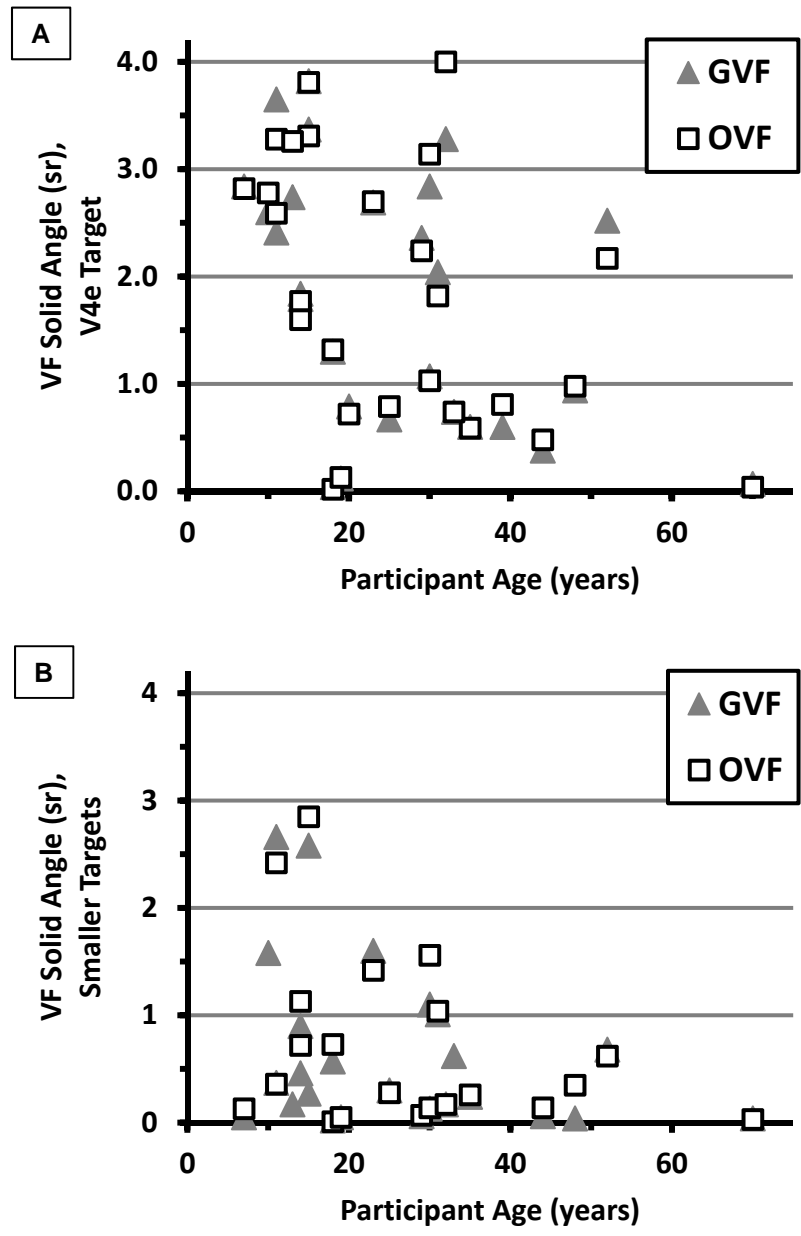
Supplementary Figure 2: Solid-angle measures, averaged across visits, as a function of participant age for the V4e target (A) and the smaller targets (B). The Goldmann visual field (GVF) results are represented by triangles and the Octopus visual field (OVF) results by open squares.
