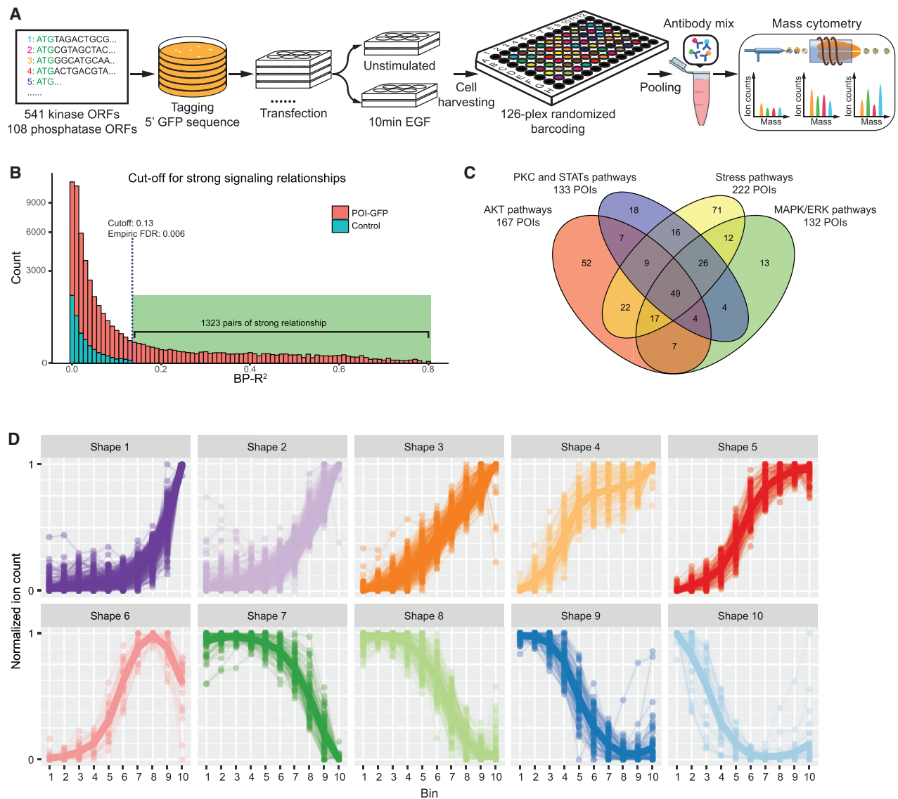
Figure 1. Kinome- and Phosphatome-wide Screen for Effects of Protein Abundance on Signaling States and Dynamics
