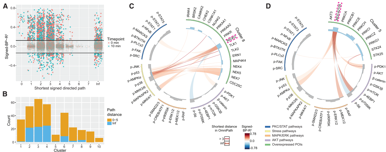
Figure 4. Prediction of Potential Signaling Connections by Comparison with Literature Evidence in the Signaling Interaction Database OmniPath
