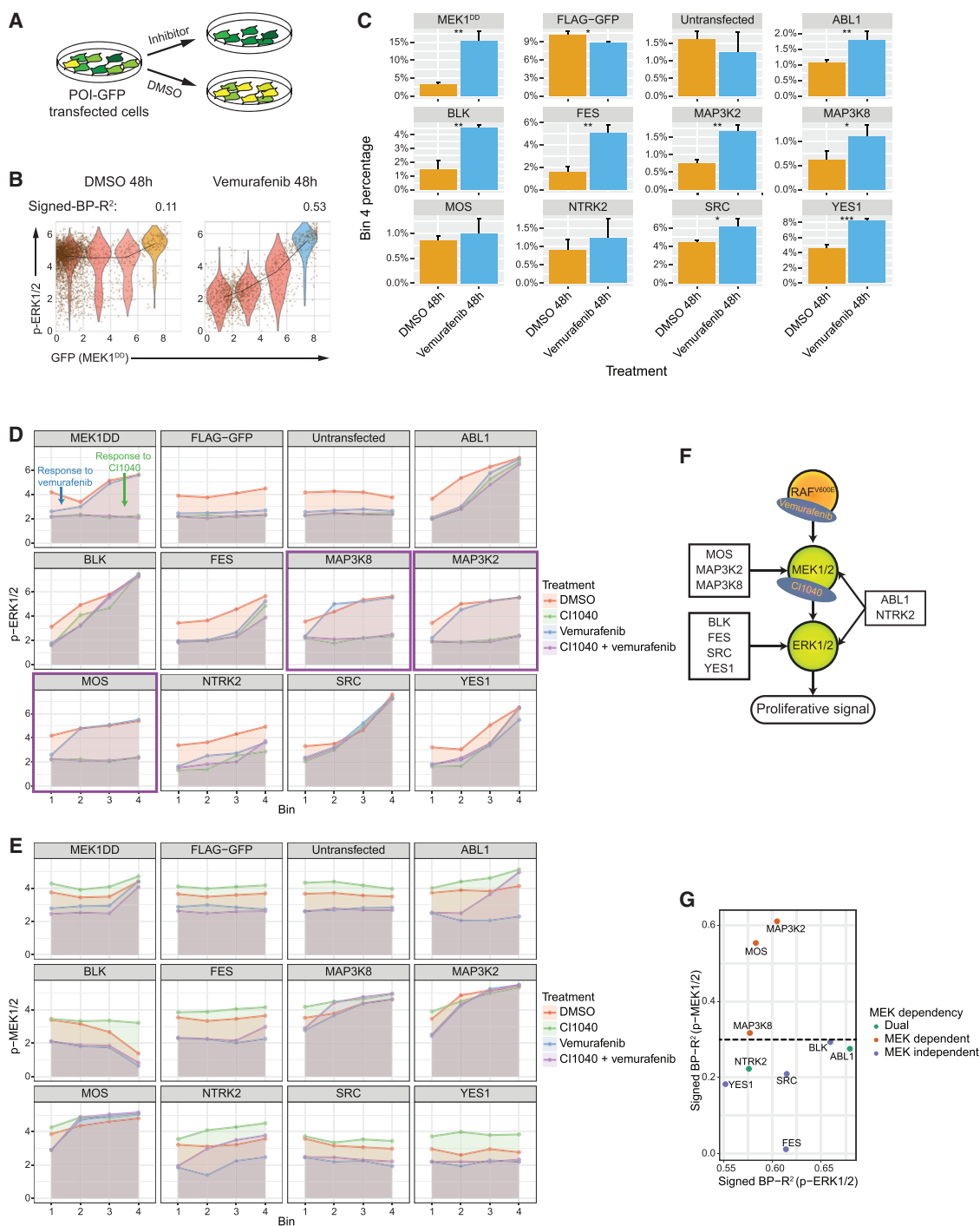
Figure 7. Kinase Overexpression Induces Resistance to BRAF-MEK Concurrent Inhibition in Melanoma Cells by MEK-Independent ERK Reactivation
