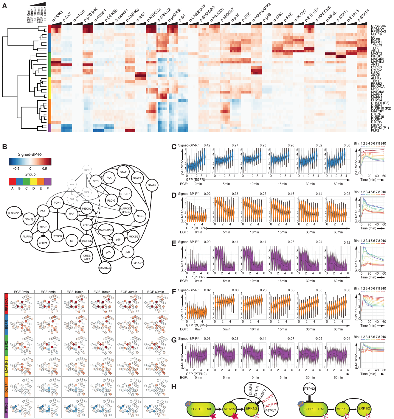
Figure 5. Effects of EGF Stimulation on 39 Kinases and Phosphatases
