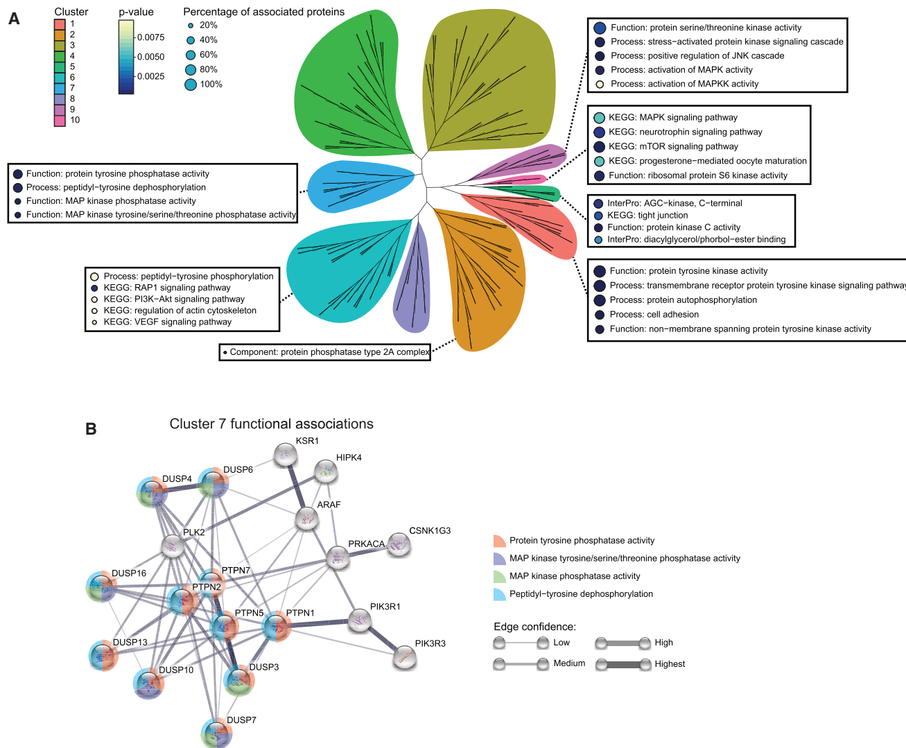
Figure 3. Functional Enrichment Analysis of Kinases and/or Phosphatases in Each Cluster
