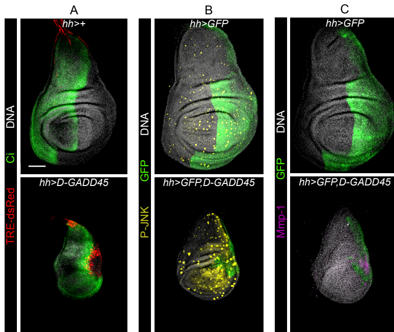
Figure S1. Sustained expression of D-GADD45 activates JNK. Detection of JNK activity using the reporter line TRE-dsRed (A) and two different markers, P-JNK (B) and Mmp-1 (C). Green: anterior compartment (A), posterior compartment (B-C), white: DNA, red: TRE-dsRed, yellow: P-JNK and magenta: Mmp-1. Bar: 50 \mu m. N \geq 5 for each genotype
