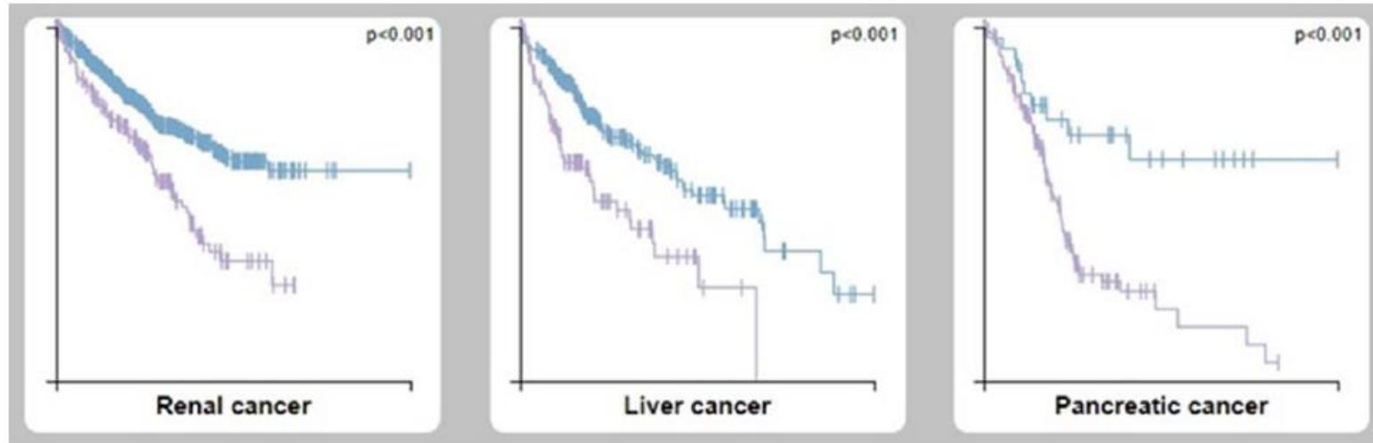
Figure S1. Pathology aspect of DCLRE1B gene. Significant association ( p < 0.01 ) with patient survival rate between cancers and high expression of DCLRE1B are shown as Kaplan-Meier plots using pathology data from protein atlas (v17.proteinatlas.org). In renal, liver and pancreatic cancer, prognosis shows as unfavourable. Whether the prognosis is favourable or unfavourable is indicated in brackets.
