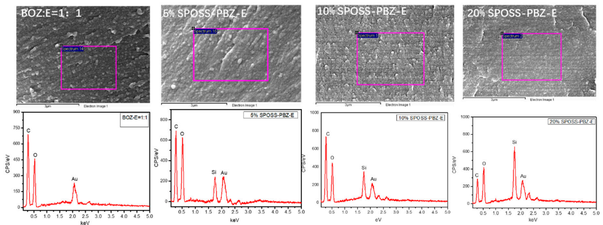
Figure S3. EDX analysis of the fracture surface of SPOSS-PBZ-E.
