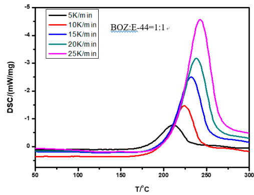
Figure S1. The DSC curves of benzoxazine at different heating rates.
