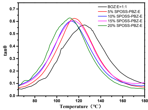
Figure S2. Tan \delta curves of nanocomposites containing various SPOSS-BOZ contents.
