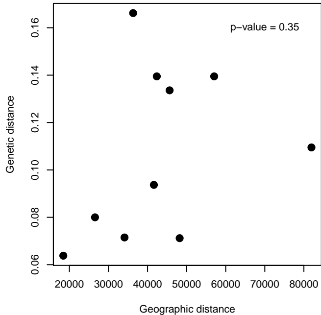
C. darwiniana
