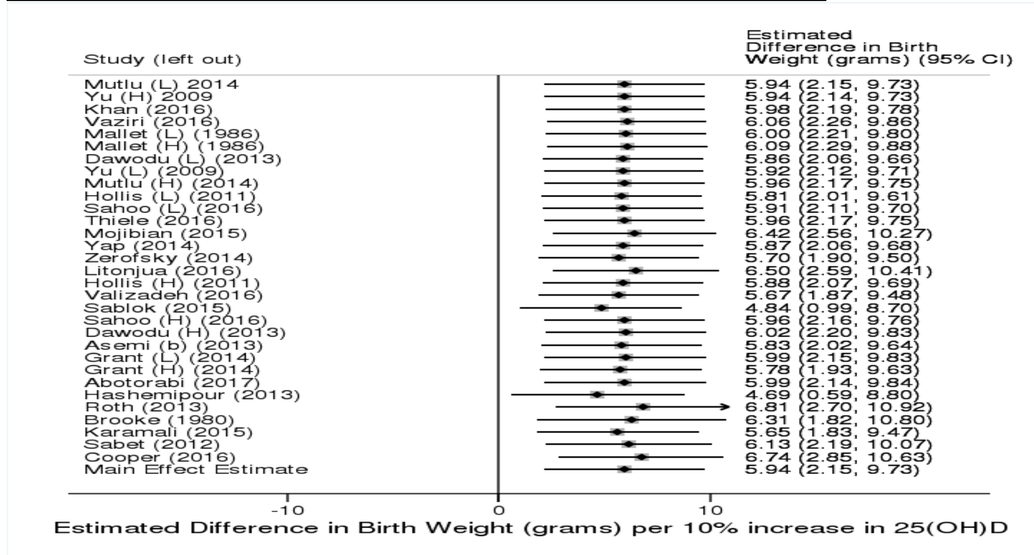
S5 Fig: Leave-One-Out Analysis for effect of 25(OH)D on birth weight RCT instrumental variable Wald ratio estimate
