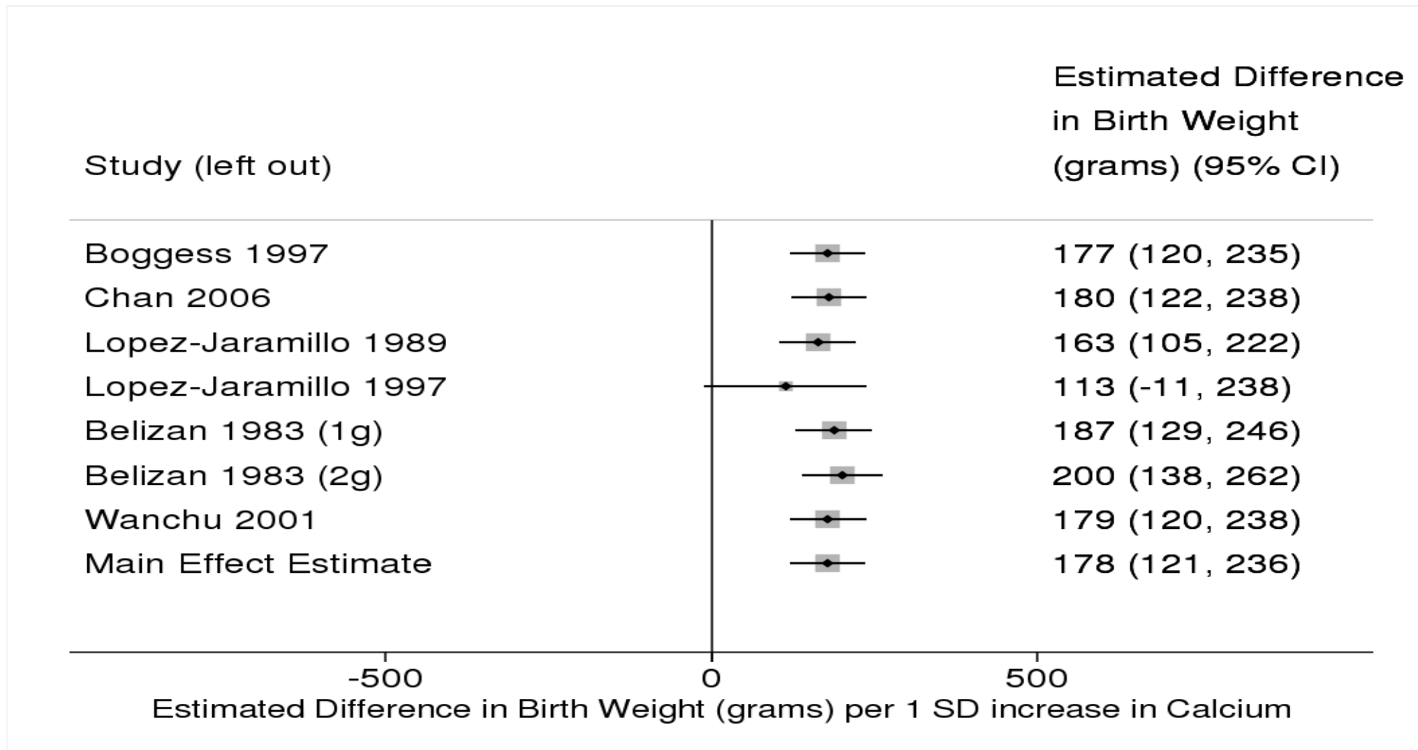
S8 Fig: Leave-One-Out Analysis for effect of maternal gestational circulating calcium RCT instrumental variable Wald ratio estimate
