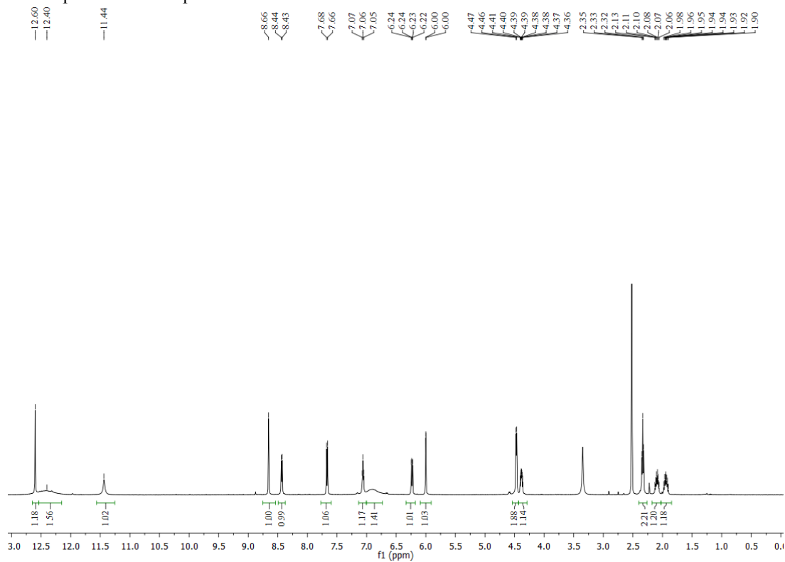
Data S2. NMR spectra of compound 3, Related to STAR methods. (top) ^1\text{H} NMR of compound 3, (bottom) ^{13}\text{C} NMR spectrum of compound 3.
